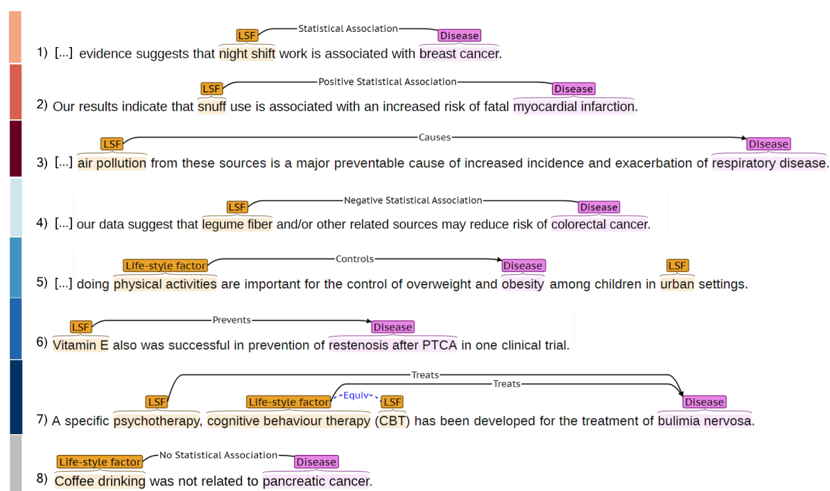
Figure 1. Illustration of the eight LSF–disease relation types in LSD600. Each line and associated color corresponds to a different type of relation: (1) Statistical Association , (2) Positive Statistical Association , (3) Causes , (4) Negative Statistical Association , (5) Controls , (6) Prevents , (7) Treats , and (8) No Statistical Association . For each relation type, we show an example as it looks in the BRAT RapidAnnotation Tool.
