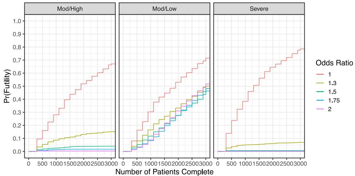
Figure 3.3.9: Effective in Severe and Moderate/High Subgroups, Cumulative Futility
