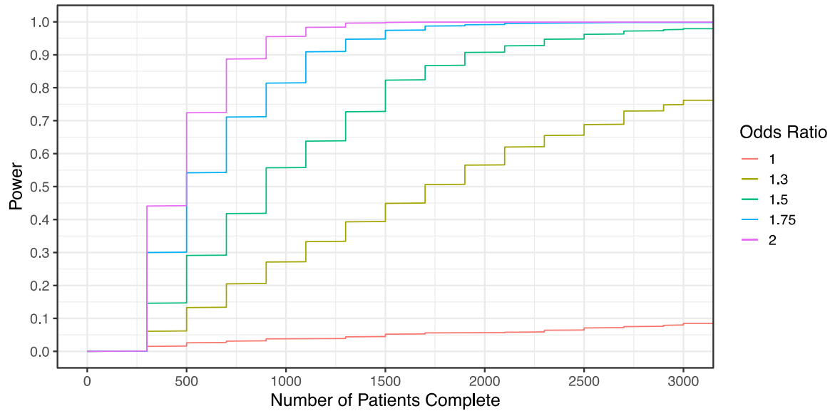
Figure 3.2.4: Effective in Severe Subgroup, Cumulative Power
