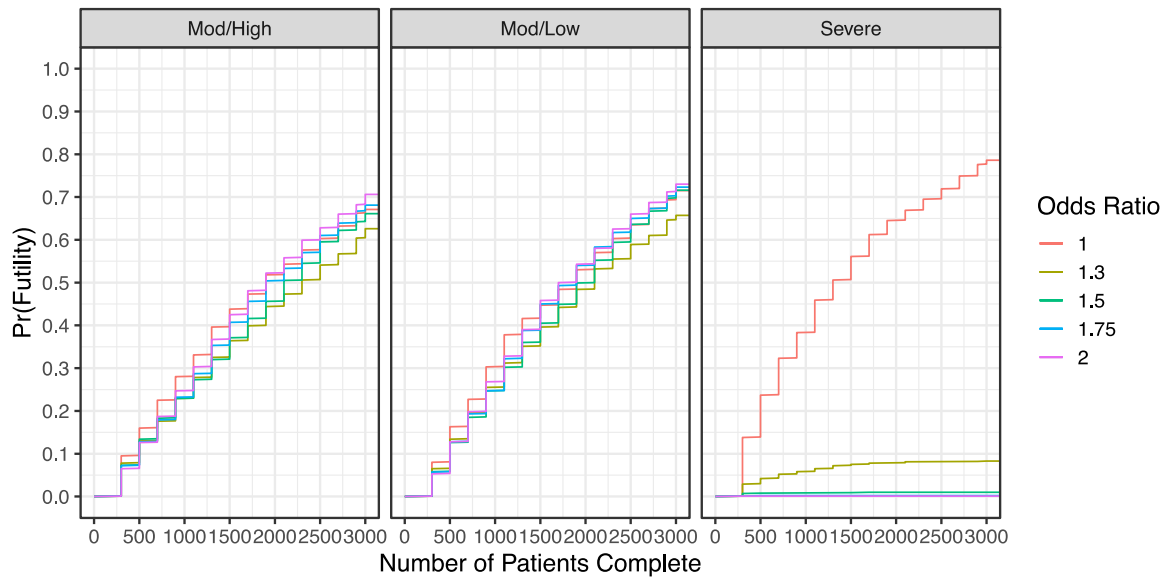
Figure 3.2.6: Effective in Severe Subgroup, Cumulative Futility
