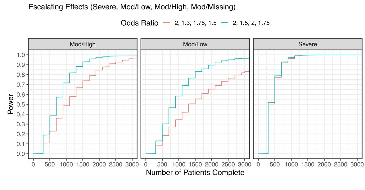
Figure 3.4.12: Escalating Effects Across Subgroups, Cumulative Futility
