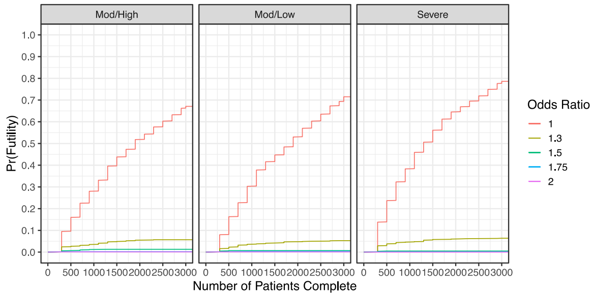
Figure 3.1.3: Same Treatment Effect Across Subgroups, Cumulative Futility
