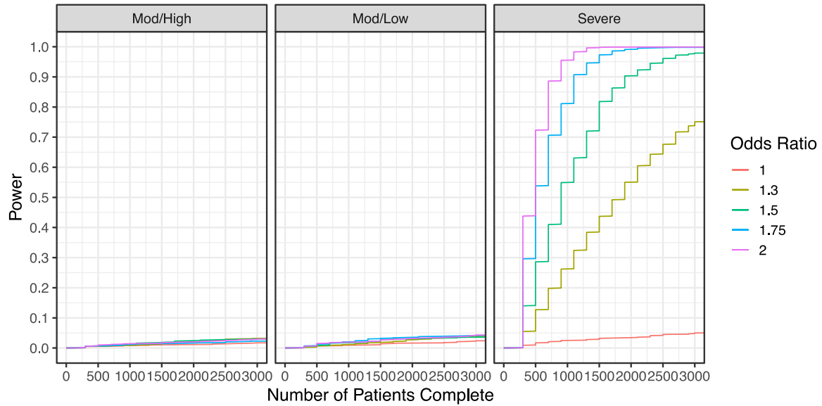
Figure 3.2.5: Effective in Severe Subgroup, Cumulative Power by Subgroup
