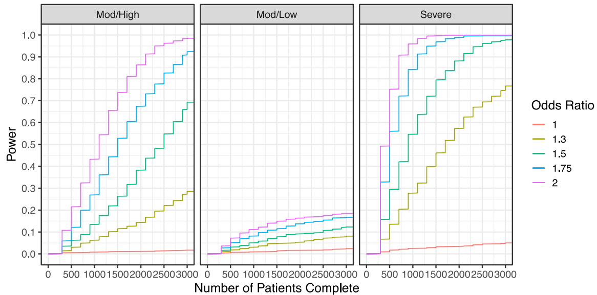
Figure 3.3.8: Effective in Severe and Moderate/High Subgroups, Cumulative Power by Subgroup
