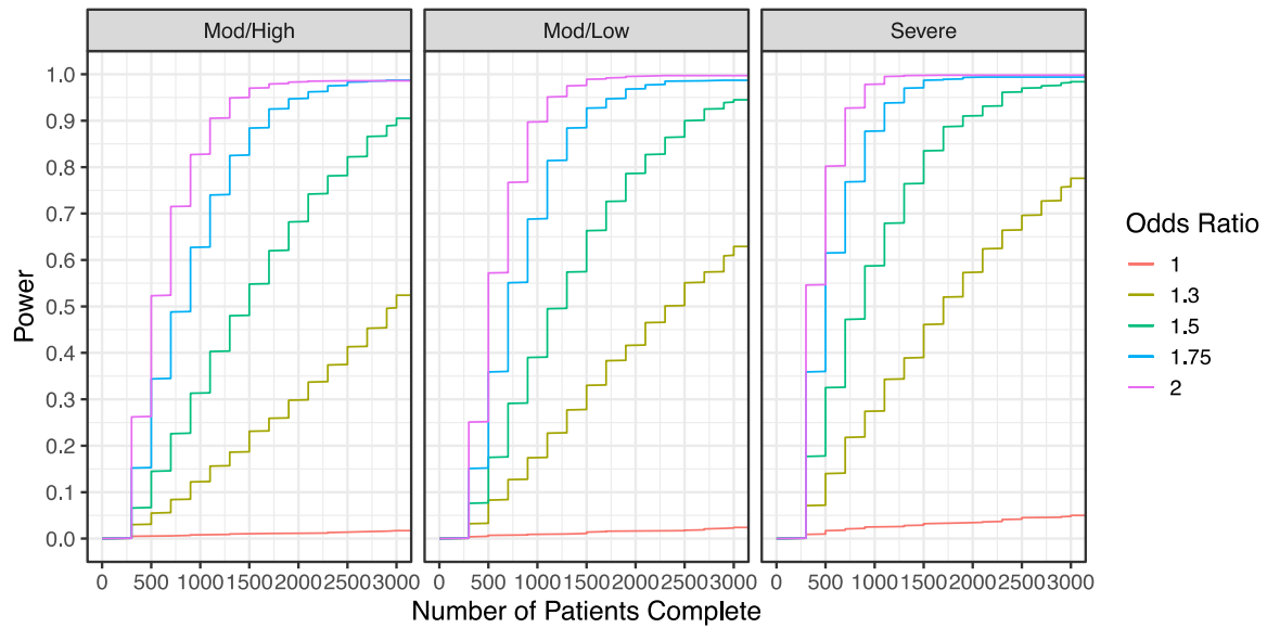
Figure 3.1.2: Same Treatment Effect Across Subgroups, Cumulative Power by Subgroup
