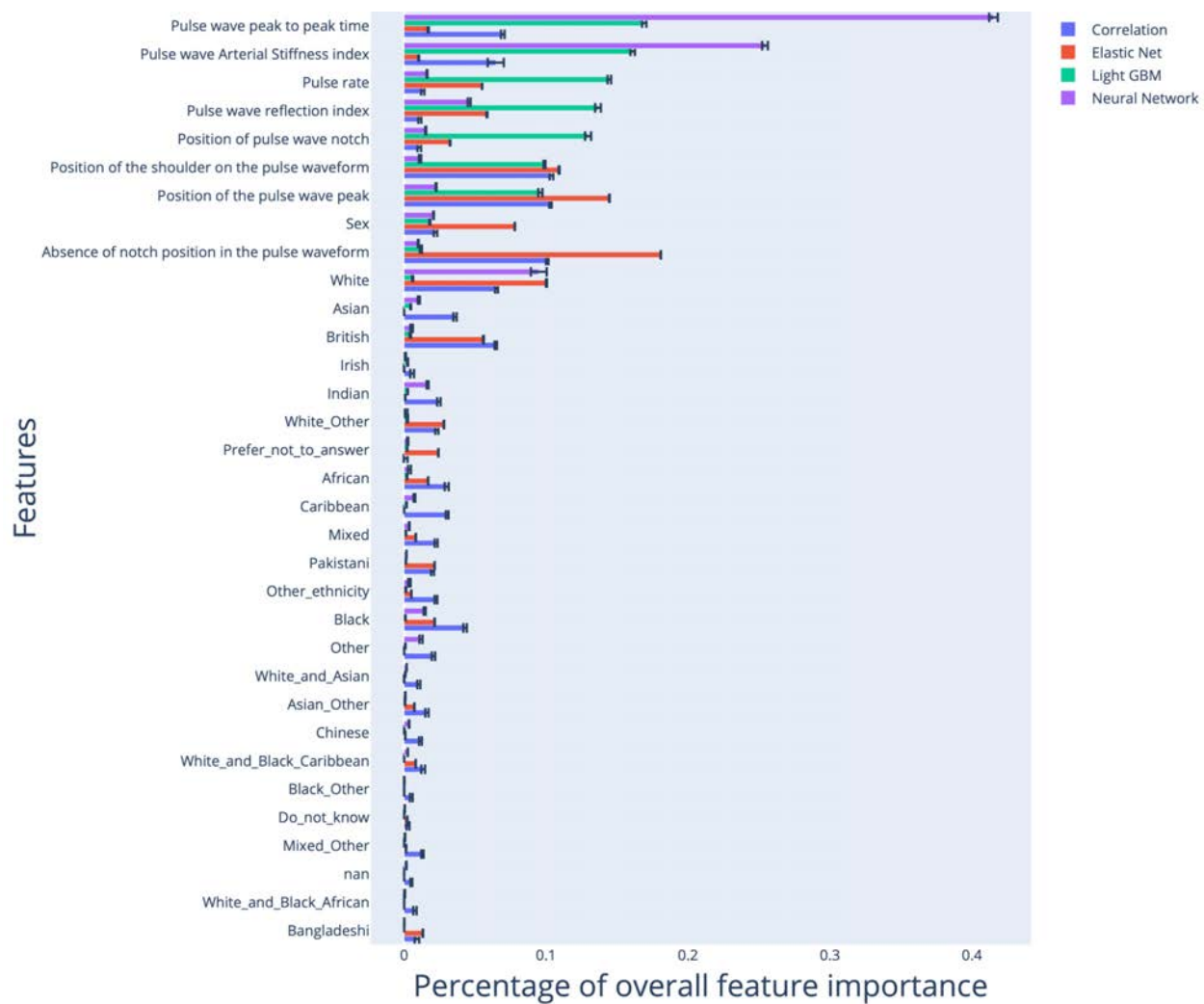
Figure S5: Feature importances for the model built on pulse wave analysis scalar features
