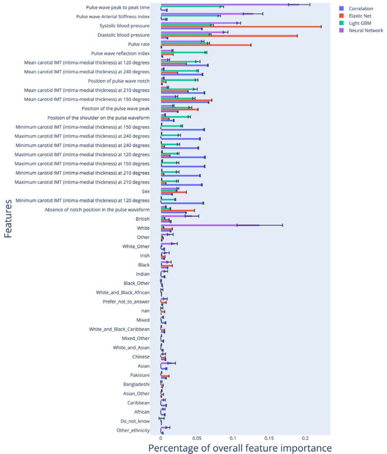
Figure S3: Feature importances for the model built on all scalar features
