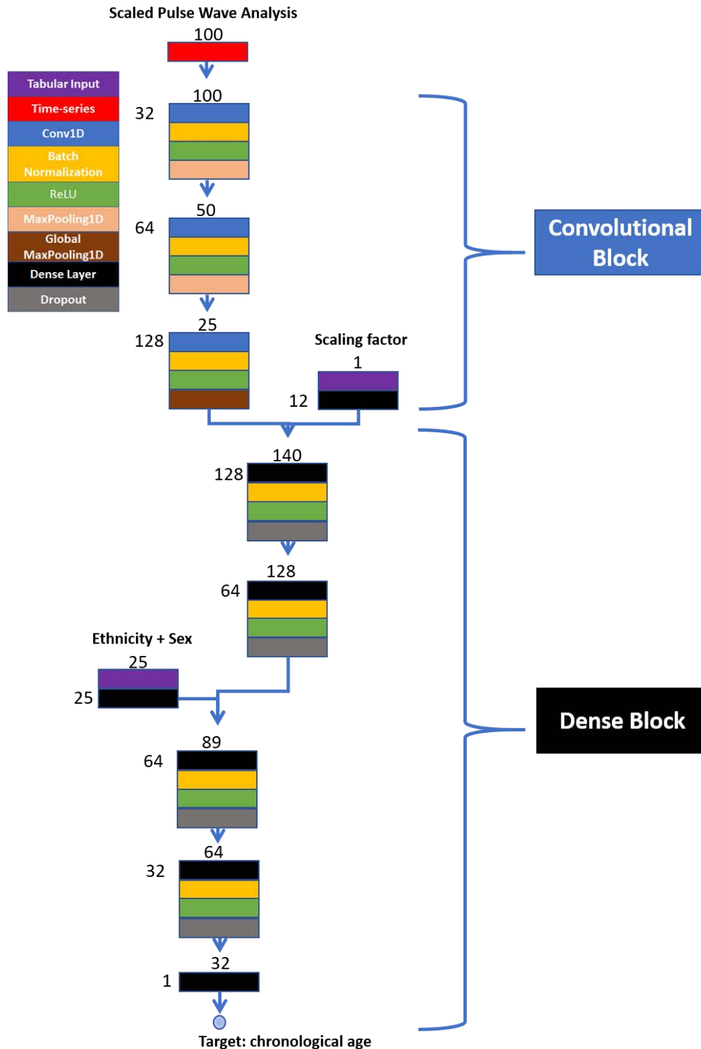
Supplementary Figure 70: Architecture of the convolutional neural network trained on pulse wave analysis records to predict chronological age - Summary figure
