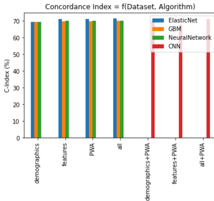
Figure S10: Survival prediction performances
