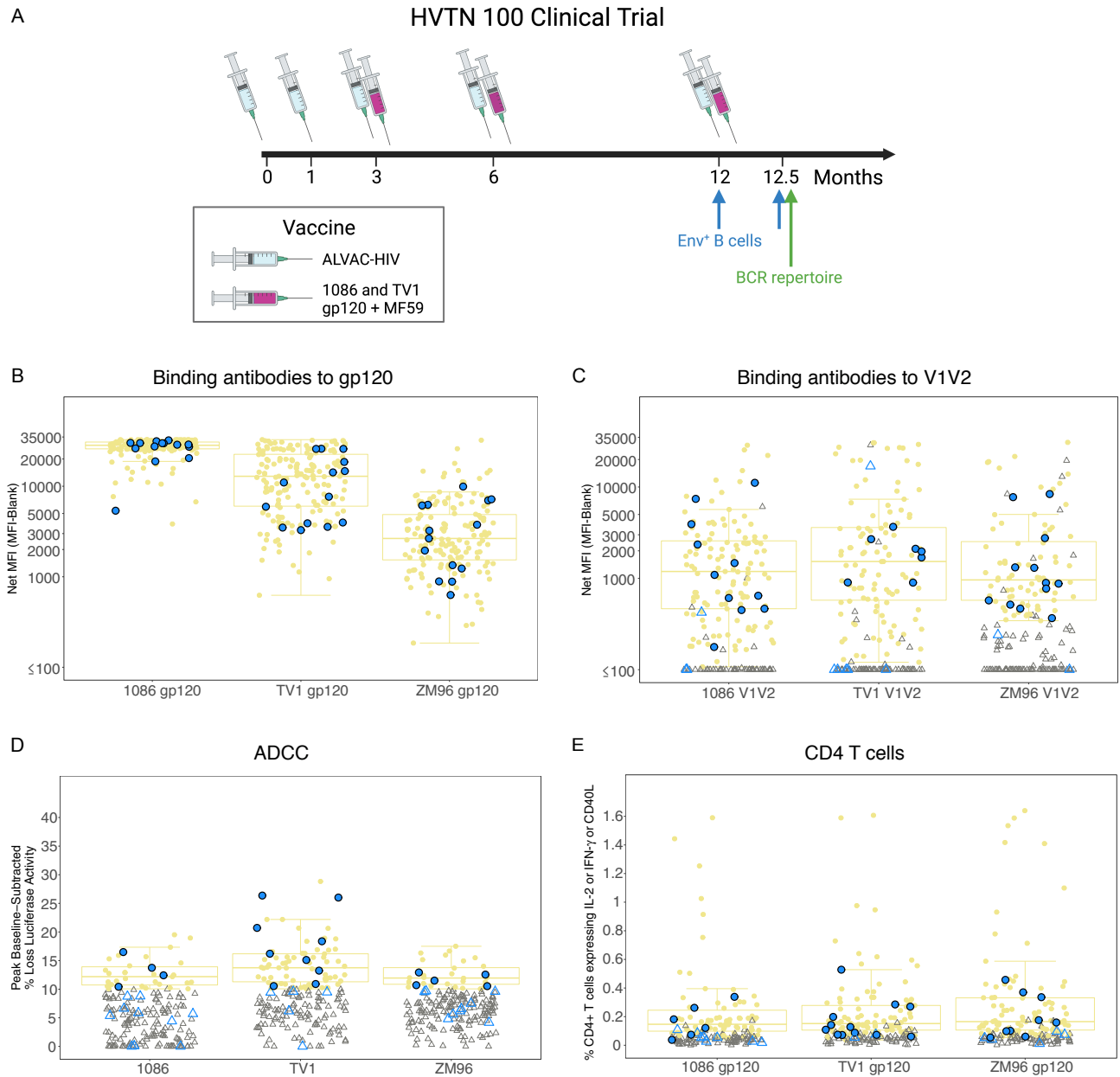
Figure S1. HVTN 100 clinical trial and immunogenicity data at month 12.5. A) Trial schema for the HVTN 100 clinical trial indicating the vaccination schedule and Env-specific B cell phenotyping and BCR repertoire analysis timepoints. Immune responses at month 12.5 to vaccine-matched antigens for the B cell analysis subset (n=14) in blue overlaid on the entire vaccinated cohort in yellow (n=185): Binding antibody responses to vaccine-matched B) gp120 and C) V1V2 proteins. D) Antibody-dependent cellular cytotoxicity (ADCC) activity of serum as measured by luciferase-based cytotoxicity assay. E) CD4 T cell responses (IL-2, IFN- \gamma , or CD40L) to vaccine-matched gp120 peptide pools. Colored circles indicate statistically “positive” response whereas open triangles indicate non-response.
