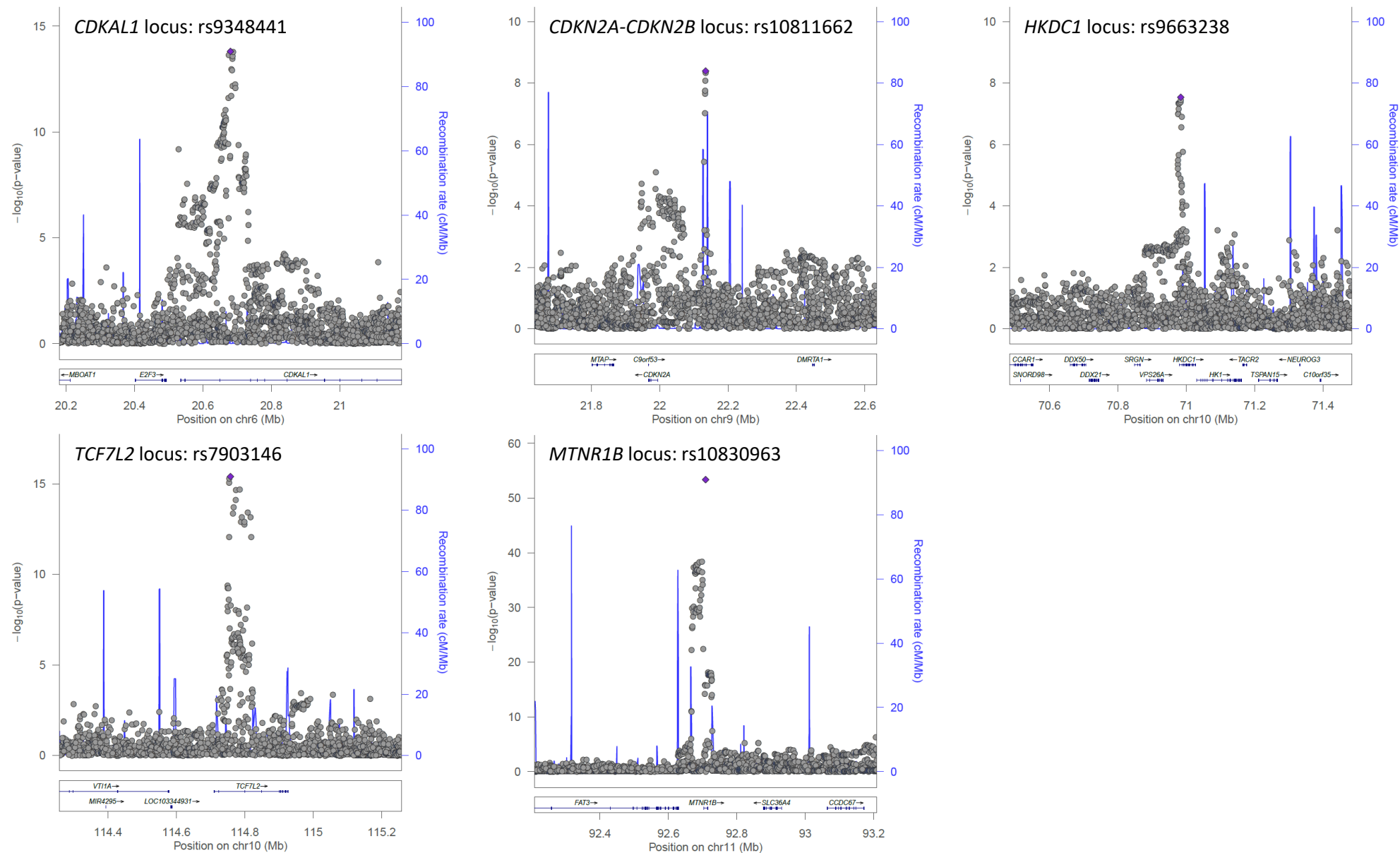
Figure S3. Signal plots for association signals with GDM at loci attaining genome-wide significance ( p < 5 \times 10^{-8} ) in trans-ancestry meta-regression (MR-MEGA) of up to 5,485 cases and 347,856 controls. Each point represents a SNV passing quality control in the trans-ancestry meta-regression, plotted with their conditional p -value (on a -\log_{10} scale) as a function of genomic position (NCBI build 37). The lead SNP is highlighted with the purple diamond. Gene annotations are taken from the University of California Santa Cruz genome browser. Recombination rates are estimated from the Phase II HapMap.
