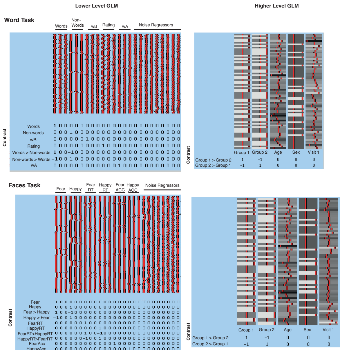
Supplementary Figure 2 – An illustration of the generalised linear models (GLM) used for both lower and higher level analyses for the word and faces task. Abbreviations as follows – wB – breathlessness rating, wA – breathlessness anxiety rating, RT – reaction time, ACC – accuracy.
