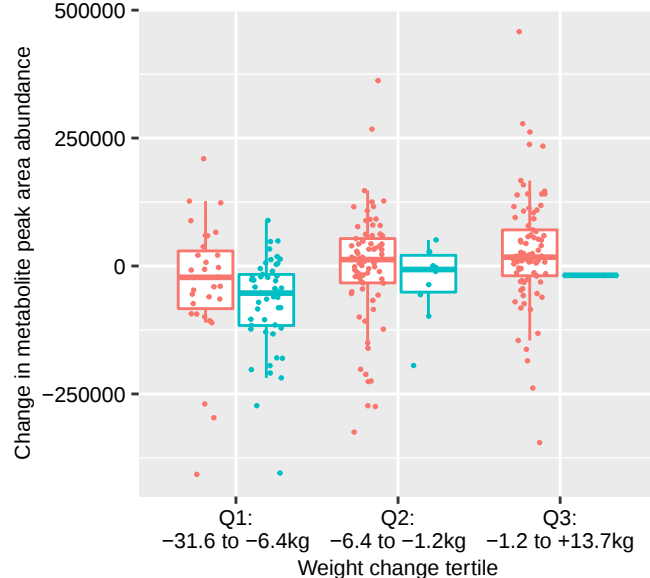
alanine
