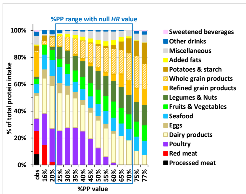
Fig. S3. Relative contribution of food categories to protein intake (in % of total protein intake) in the observed diets (obs) and modeled diets obtained by long-term health risk ( HR ) and diet departure minimization under imposed percentage of plant protein in the diet (%PP) in French adults. Results are reported for all the adequate %PP values ensuring nutrient adequacy and model convergence, of which only the 25%-70% range ensured a null HR value. See Supplemental Table 5 for the detailed composition of food categories.
