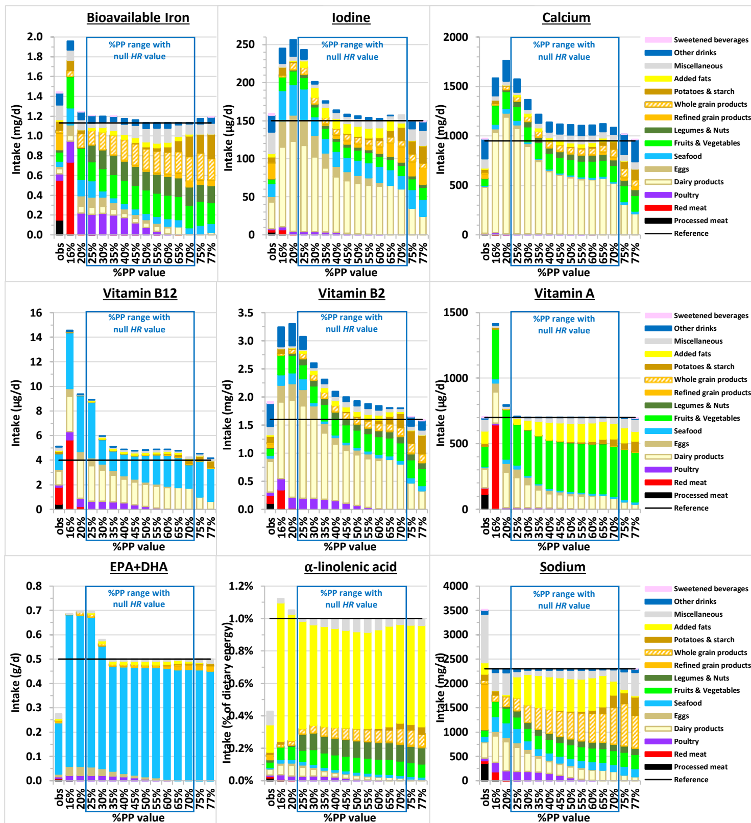
Fig. S4. Contribution of food categories to intakes of nutrients that are limiting for a high plant protein percentage in the diet (%PP \geq 75%) in observed (obs) and modeled diets obtained by long-term health risk ( HR ) and diet departure minimization under imposed %PP value in French adults. Results are reported for all the adequate %PP values ensuring nutrient adequacy and model convergence, of which only the 25%-70% range ensured a null HR value. The line represents the constraint for the selected nutrient (lower bound, except for sodium that is upper bound). For bioavailable iron and vitamin A, constraints are represented as the mean between the constraint for males and females. For other nutrients, constraints are similar between sexes. See Supplemental Table 7 for the detailed values of the constraints, and Supplemental Table 5 for the detailed composition of food categories.
