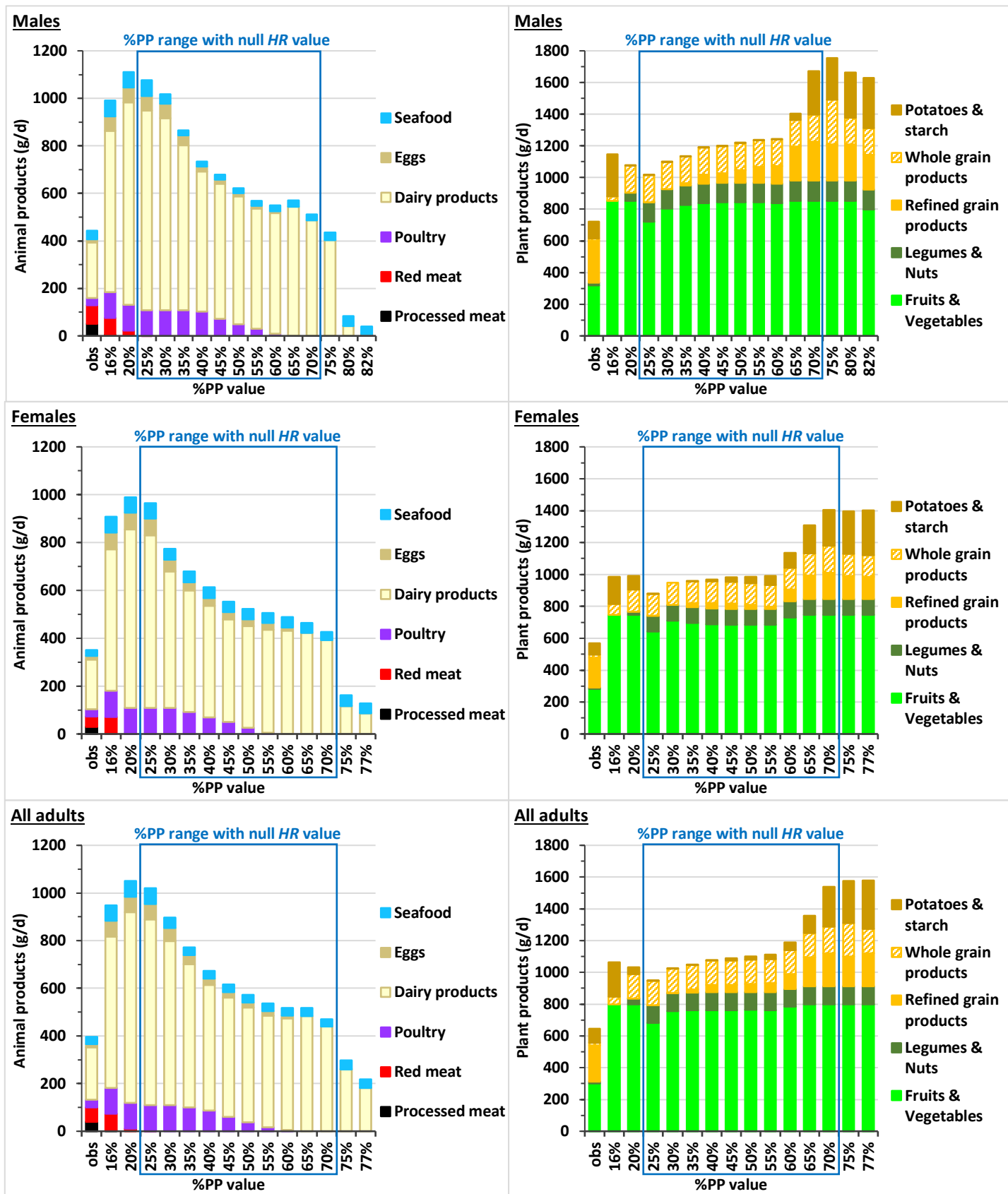
Fig. S2. Daily food category consumption in the observed diets (obs) and modeled diets obtained by long-term health risk ( HR ) and diet departure minimization under imposed percentage of plant protein in the diet (%PP) in French males, females and all adults. Results are reported for all the adequate %PP values ensuring nutrient adequacy and model convergence, of which only the 25%-70% range ensured a null HR value. The bar charts represent cumulative consumption of the main animal-based or plant-based food categories. Details about food grouping and consumptions of food categories not shown here are given in Supplemental Tables 5 and 2, respectively.
