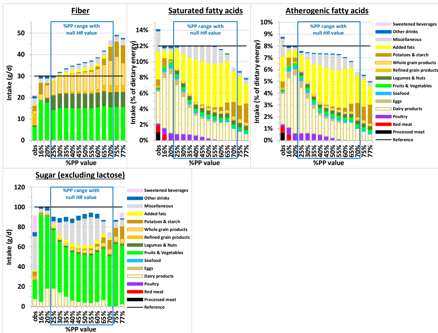
Fig. S5. Contribution of food categories to the intakes of nutrients that are limiting for a low plant protein percentage in the diet ( \%PP \leq 20\% ) in observed (obs) and modeled diets obtained by long-term health risk ( HR ) and diet departure minimization under imposed \%PP value in French adults. Results are reported for all the adequate \%PP values ensuring nutrient adequacy and model convergence, of which only the 25%-70% range ensured a null HR value. The line represents the constraint for the selected nutrient (upper bound, except for fiber that is lower bound). See Supplemental Table 5 for the detailed composition of food categories. Atherogenic fatty acids, lauric and myristic and palmitic acids.
