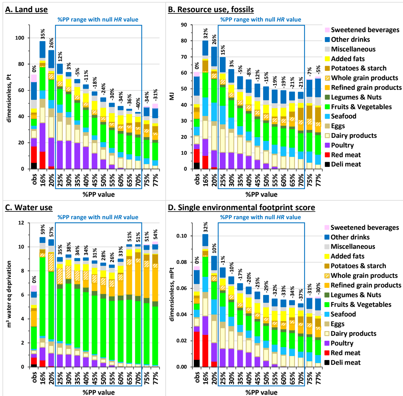
Fig. S6. Land use (A), fossils resource use (B), water use (C) and single environmental footprint score aggregating 16 indicators (D) associated with the observed (obs) and modeled diets obtained by long-term health risk ( HR ) and diet departure minimization under imposed percentage of plant protein in the diet (%PP) in French adults. Results are reported for all the adequate %PP values ensuring nutrient adequacy and model convergence, of which only the 25%-70% range ensured a null HR value. Sections inside the bars represent the contributions of food categories to the considered environmental indicator, and values above the bars represent the percentage deviation in the environmental indicator from its observed value. See Supplemental Table 5 for the detailed composition of food categories.
