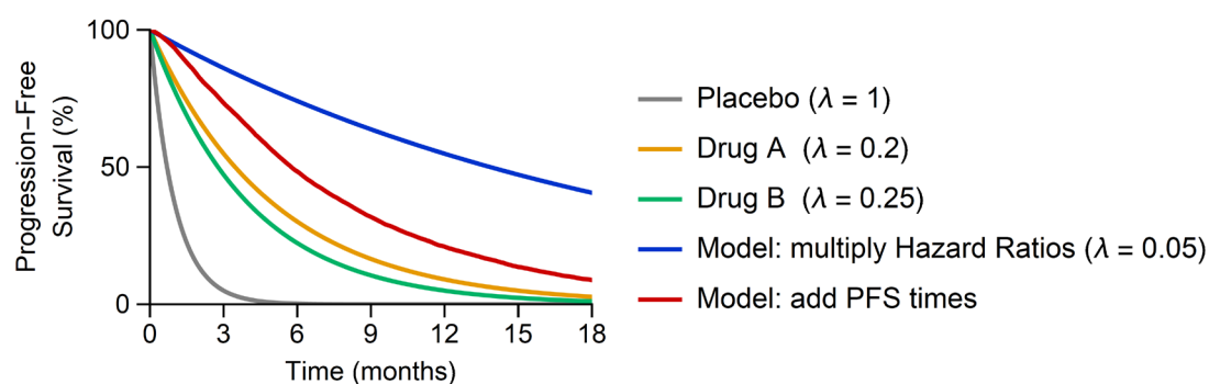
Figure S2. Multiplying Hazard Ratios results in unrealistic predictions with survival times that are far longer than arithmetic addition. Exponential survival functions were simulated with rate parameters of \lambda = 1, 0.2 , and 0.25 , for placebo, drug A, and drug B, respectively. The effects of an 'additive' combination were simulated by the addition of PFS times (the model proposed in this study, using correlation \rho = 0.3 and scan interval 1.5 months), or by multiplying the hazard ratios of single drugs relative to placebo, which results in a rate of \lambda = 0.05 . Median PFS time from multiplying hazard ratios is four times as large as the most active single drug (14 months vs. 3.5 months), making it much more than the addition of single drug PFS times.
