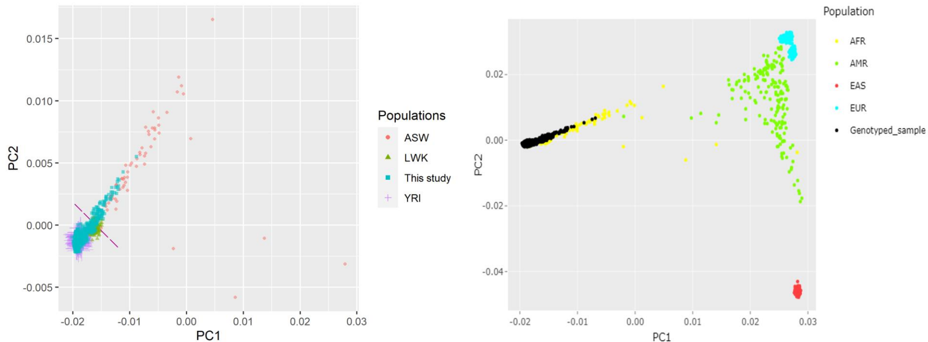
Supplementary Figure 1. (a) The principal component analysis shows individuals from the Southern Nigeria (below the dashed line) and those from the Northern Nigeria (above the dashed line). YRI: Yoruba in Ibadan population; LWK: Luhya in Webuye, Kenya; ASW: Americans of African Ancestry in Southwest USA. (b). The principal component analysis of the Nigerian cohort alongside the major population ancestries. AFR: Africa; AMR: America; EAS: East Asia; EUR: Europe.
