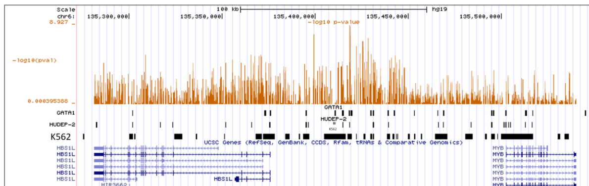
Supplementary Figure 3: UCSC plot for the HMIP locus. Tracks in order: \log_{10} p-values for variants; GATA1 ChIP-seq annotation; HUDEP-2 annotation; K562 annotation; genes in this locus.
