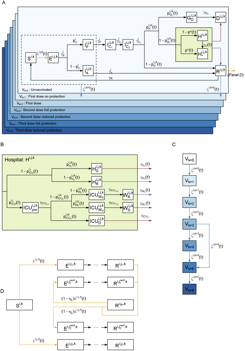
Figure S1: Model structure flow diagram with rates of transition between states. (A) Extended SEIR transmission model flow diagram overview. (B) Hospital flow diagram. (C) Vaccination flow diagram. (D) Multi-variant flow diagram. Model state variables and parameters are presented in detail throughout this supplement; in particular, see section 4.
