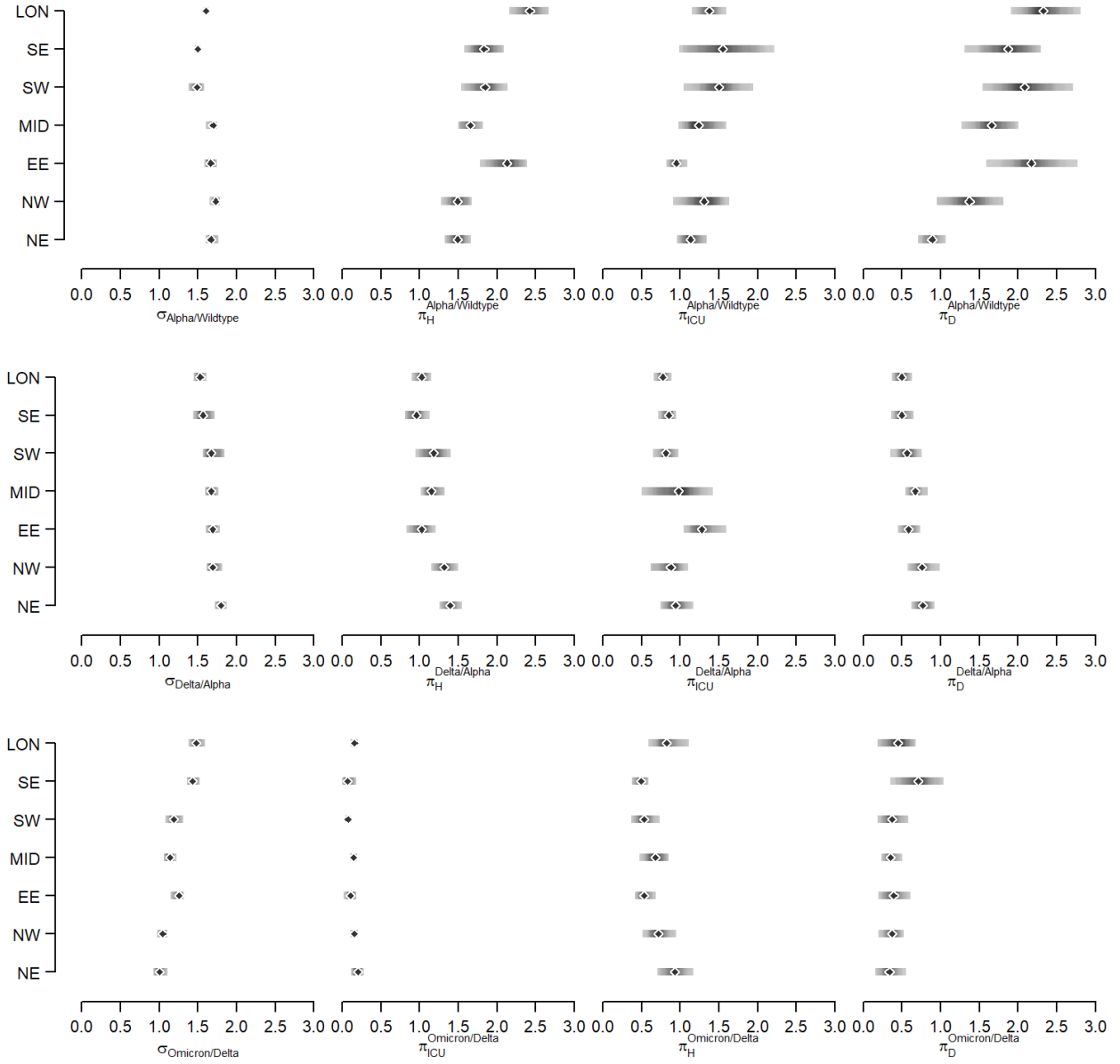
Figure S35: Model parameter posterior distributions for variant-driven severity modifiers. The points show the median model fit and the bars the 95% CrI. We assumed a uniform (flat) prior, hence no prior bounds are shown.
