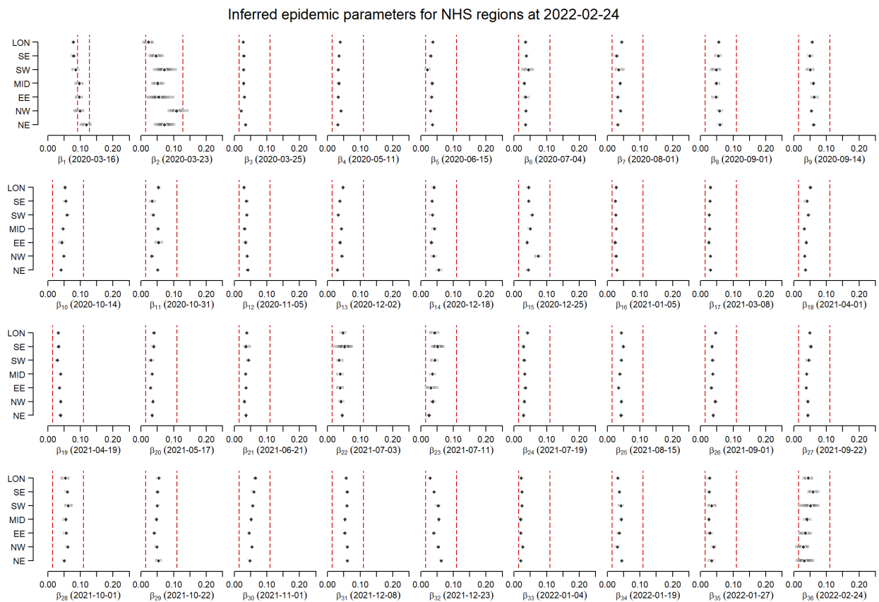
Figure S33: Estimated value of beta over time by region. The points show the median model fit and the bars the 95% CrI. The vertical dashed red lines show the bounds of the prior distribution.
