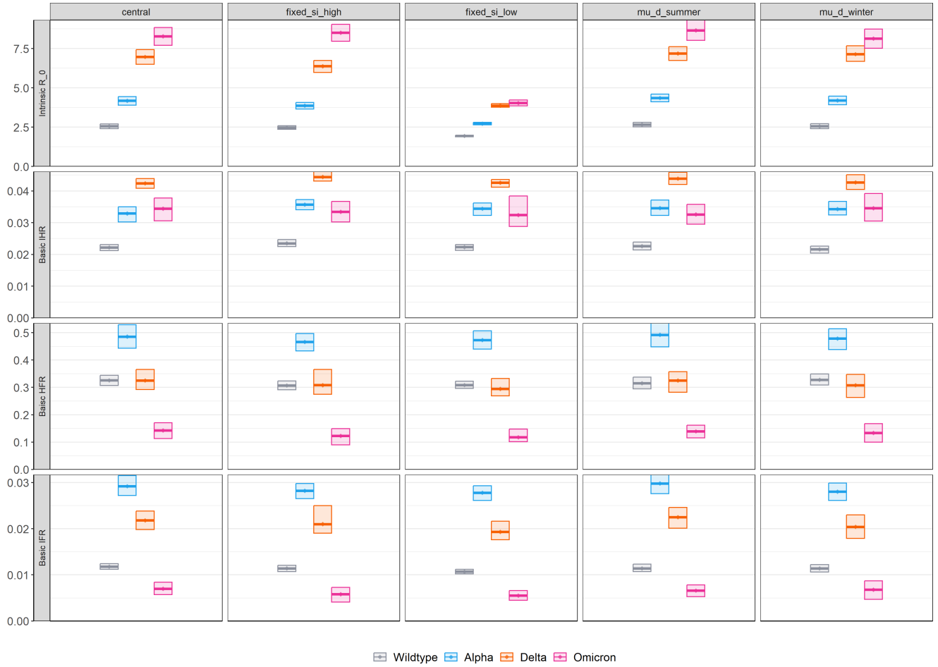
Figure S10: Sensitivity analysis of model inferred intrinsic R_0 and basic IHR, HFR and IFR of the variants. From left to right: Central, high and low fixed serial interval duration (see values in table S13), and alternative changepoints for \mu_D(t) in the winter of 2020/21 and in the summer of 2021 (see values and rationale in table S17). Box plots show mean model-inferred properties and 95% CrI for the Wildtype (grey), Alpha (blue), Delta (orange) and Omicron (pink) variants.
