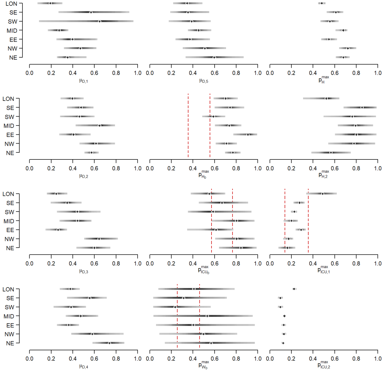
Figure S34: Model parameter posterior distributions for time-varying severity modifiers. The points show the median model fit and the bars the 95% CrI. Where shown, vertical dashed red lines show the bounds of the prior distribution, else we assumed a uniform (flat) prior.
