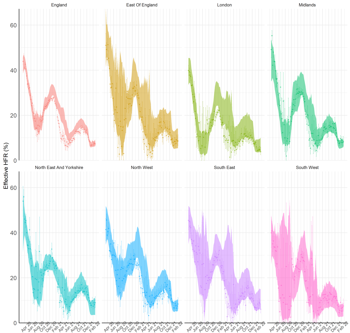
Figure S14: Point-range represents data and binomial confidence interval (see section 6.2) for details of data aggregation from linked patient-level line lists) and shaded areas 95%CrI of model inferred trajectories by NHS England region.
