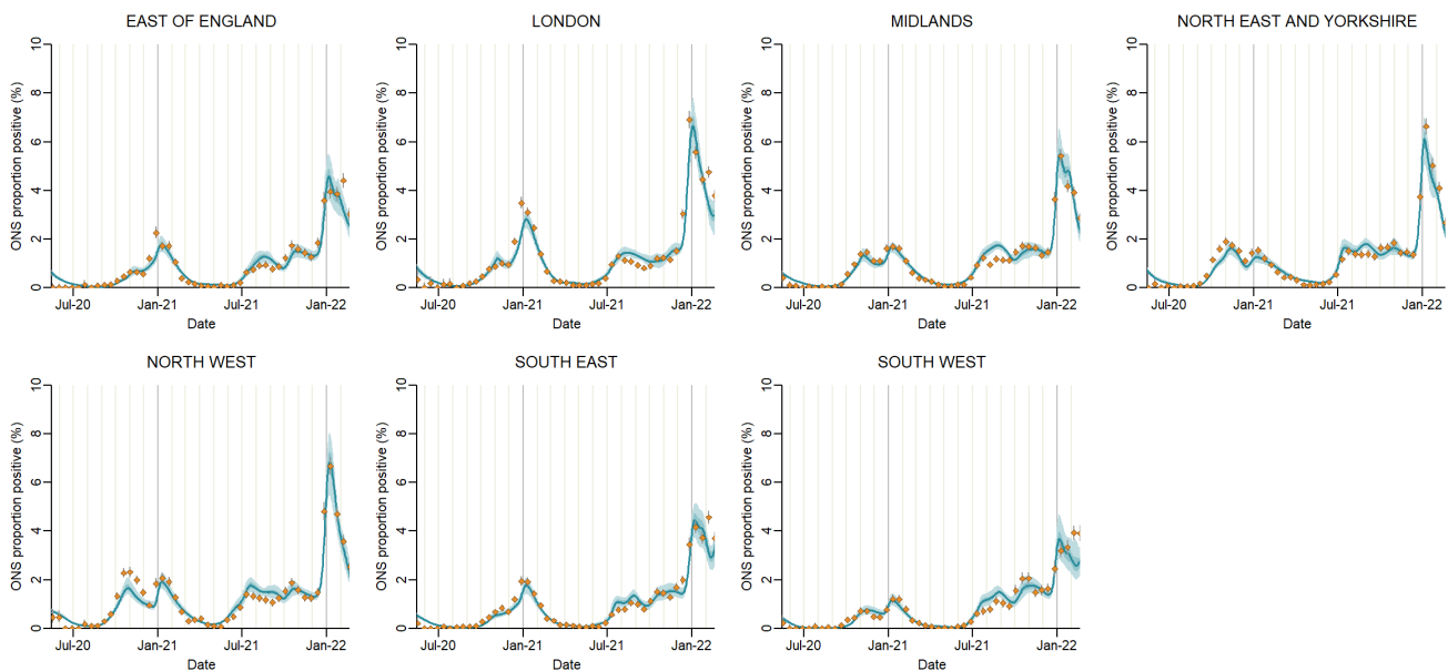
Figure S19: Model fits to NHS England Regions (columns): infection prevalence in the community from ONS infection survey. Points show the data, the solid line the median model fit and the shaded area the 95% CrI.
