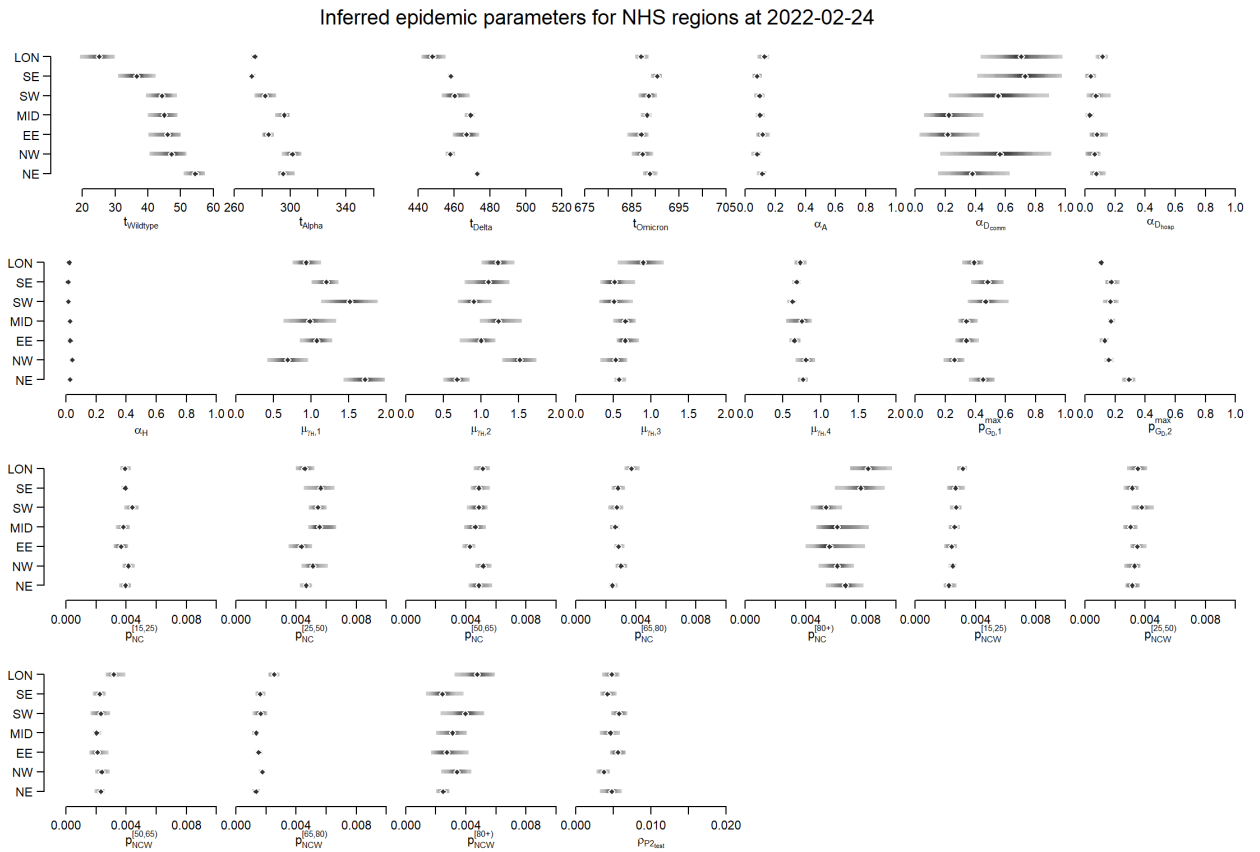
Figure S36: Model parameter posterior distributions. The points show the median model fit and the bars the 95% CrI. We assumed a uniform (flat) prior, hence no prior bounds are shown.
