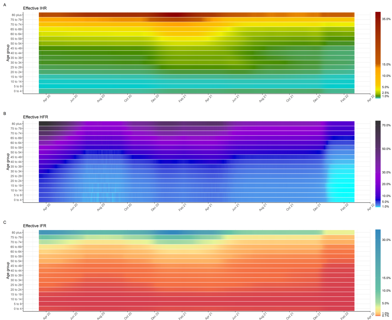
Figure S16: Effective infection hospitalisation ratio (IHR), hospital fatality ratio (HFR) and infection fatality ratio (IFR) by model age compartments over time, accounting for immunity by age class. Please note different colour gradient scales for each heatmap.
