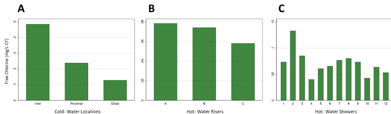
Figure S3. A) Free chlorine mean concentration across cold-water sample locations. B) Free chlorine concentration across risers from hot-water samples. C) Free chlorine concentration across 12 showers from hot-water samples.
