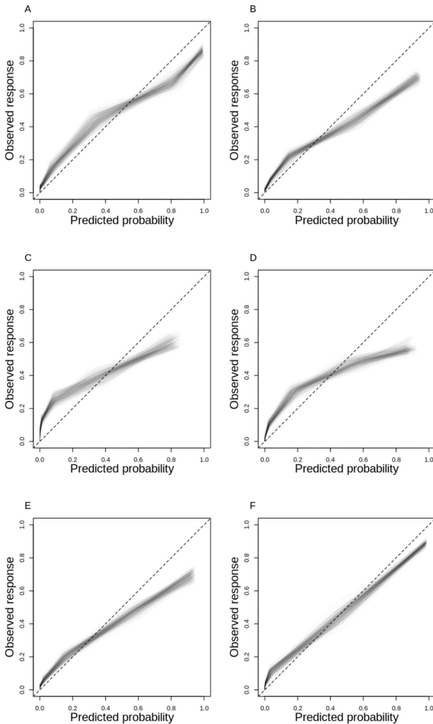
Supplementary Figure 2 A-F: Calibration plots of Bayesian Additive Regression Trees (BART) showing the goodness-of-fit between the decile of predicted probabilities and the proportion of outcomes that are: A) lying, B) sitting, C) self-paced walking, D) running at 3 METs, E) running at 5 METs, and F) running at 7 METs. Translucent lines represent the iterations of Markov Chain Monte Carlo. The x-axis indicates the decile of predicted probability, and y axis indicates the proportion of the outcome corresponding to the deciles of predicted probabilities. Panel C and D shows a larger miscalibration (discordance) between the predicted and observed outcome probabilities, with BART underestimating the outcomes when predicting low probabilities, and overestimating when predicting high probabilities. On the
