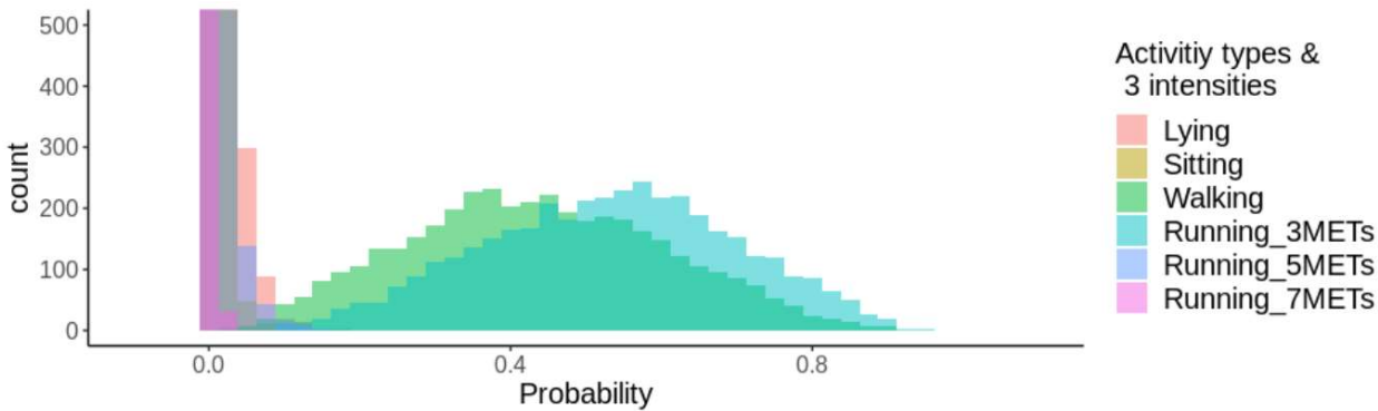
Supplementary Figure 3. Posterior predictive distribution of six activity categories at one time point, where the estimated distributions of walking and Running (3METs) are largely overlapping.
