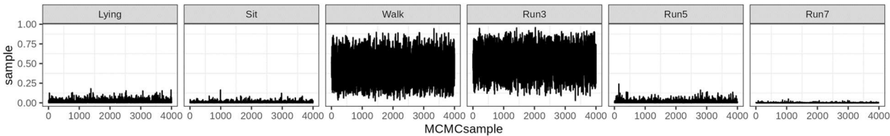
Supplementary Figure 4. Trace plots of a time point corresponding to Supplementary Figure 3 above, indicating the mixing of Markov Chain for each of the six activity categories.
