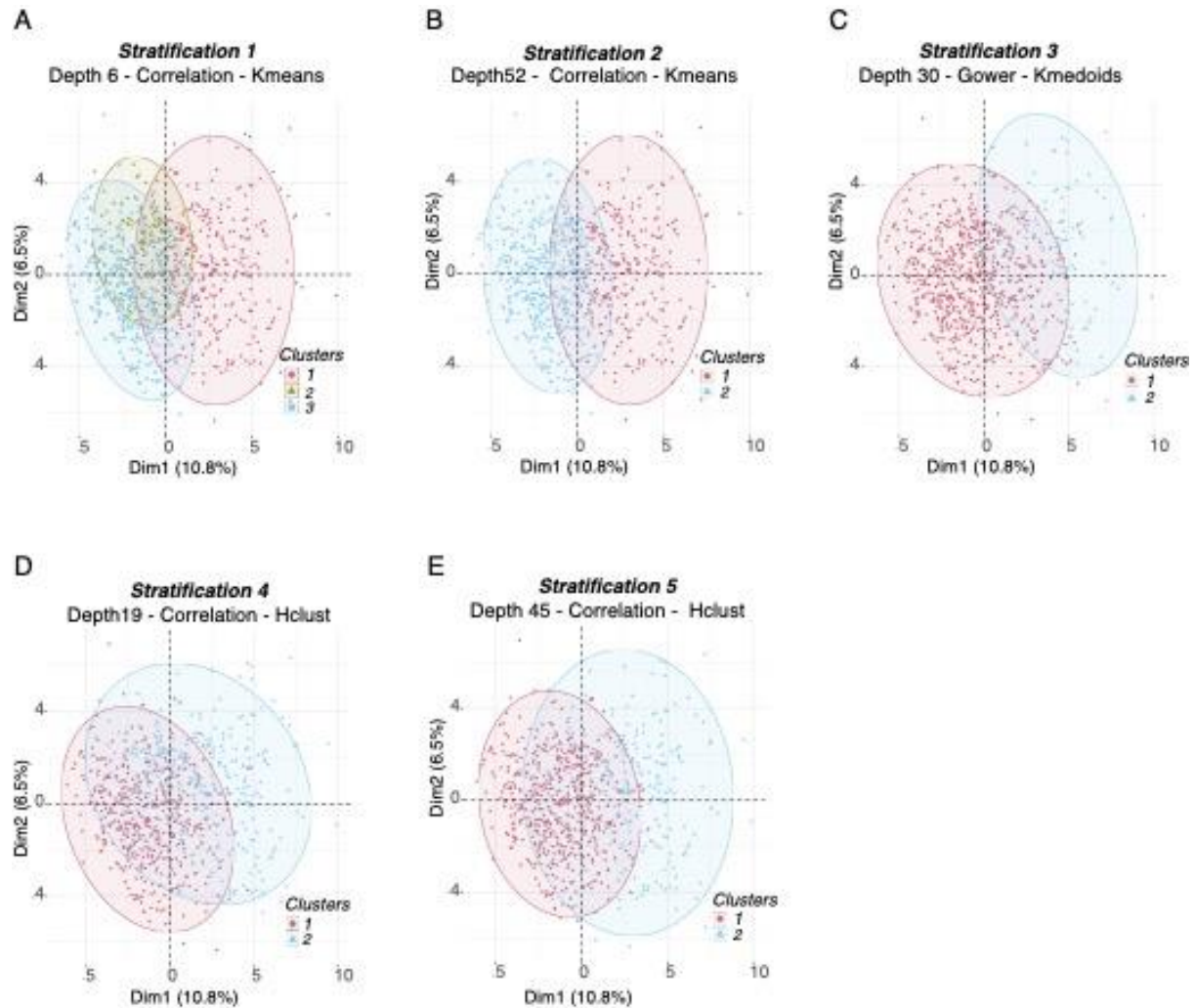
Figure S2. Principal Component projections of the ClustALL robust stratifications based on all the input variables. (A-E). Low-dimension representation of the robust stratifications after applying the ClustALL framework to the PREDICT cohort. For each one of the 5 robust stratifications identified by ClustALL, the Principal Component Analysis of all the input variables with the stratification is shown. The x (Dim1) and y (Dim2) axes represent the first and second principal components respectively, which are linear combinations of the original variables.
