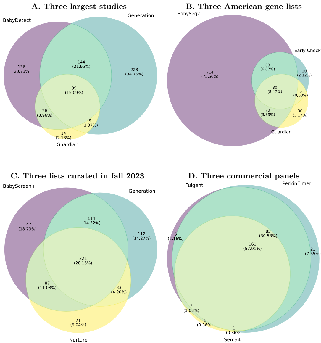
FIGURE S5: GENE LIST VENN DIAGRAMS
