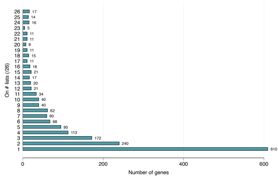
FIGURE S3: GENE INCLUSION DISTRIBUTION
