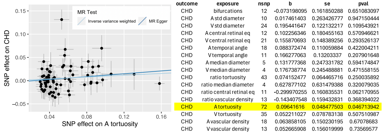
Figure 16: Results of MR analyses for arteriolar tortuosity as a causal influence on coronary heart disease (CHD) in the UKBB. Left: We were able to confirm this causal link of arterial tortuosity on CHD [48]. Fit lines correspond to inverse-variance-weighted (IVW) and Egger methods. Right: Effects from IVW for all IDPs are reported. No other retinal IDP was found to be causal.
