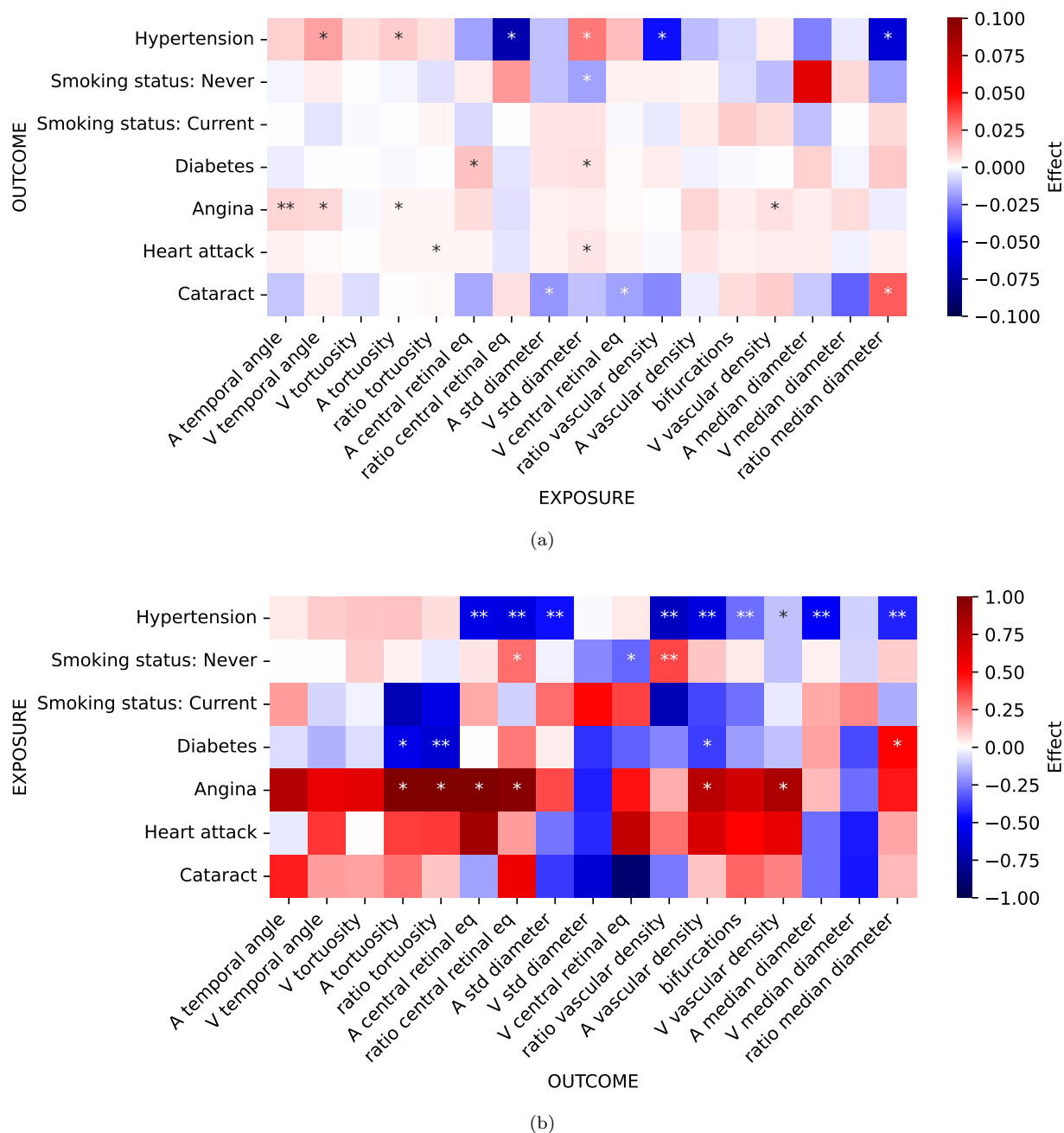
Figure 15: a) Causal effect estimates with IDPs as exposures and binary diseases as outcomes, in the UKBB. b) Causal effect estimates with binary diseases as exposures and IDPs as outcomes, in the UKBB. The color indicates the causal effect estimates based on the inverse variance-weighted MR method. The level of statistical significance is indicated with a single asterisk for nominal significance without correction for multiple testing ( * : p_{uncorrected} < 0.05 ) and two asterisks for a false discovery rate (FDR) ( ** : p_{FDR} < 0.05 ).
