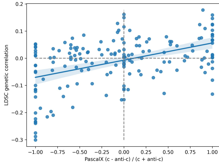
Figure 18: IDP-risk factor pairs: LDSR genetic correlation plotted against PascalX normalized coherence (number of coherent-anticoherent genes)/(number of coherent+anticoherent genes). Each dot represents a phenotype pair. The regression line is plotted with a 95% confidence interval. ‘LDSR’: Linkage Disequilibrium Score Regression, ‘c’: coherent, ‘anti-c’: anticoherent.
