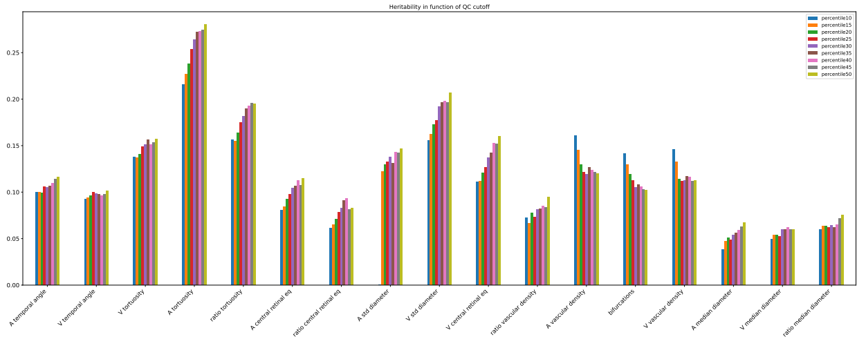
Figure 34: SNP heritabilities as a function of QC. All standard errors were smaller than 0.03, with mean=0.013
