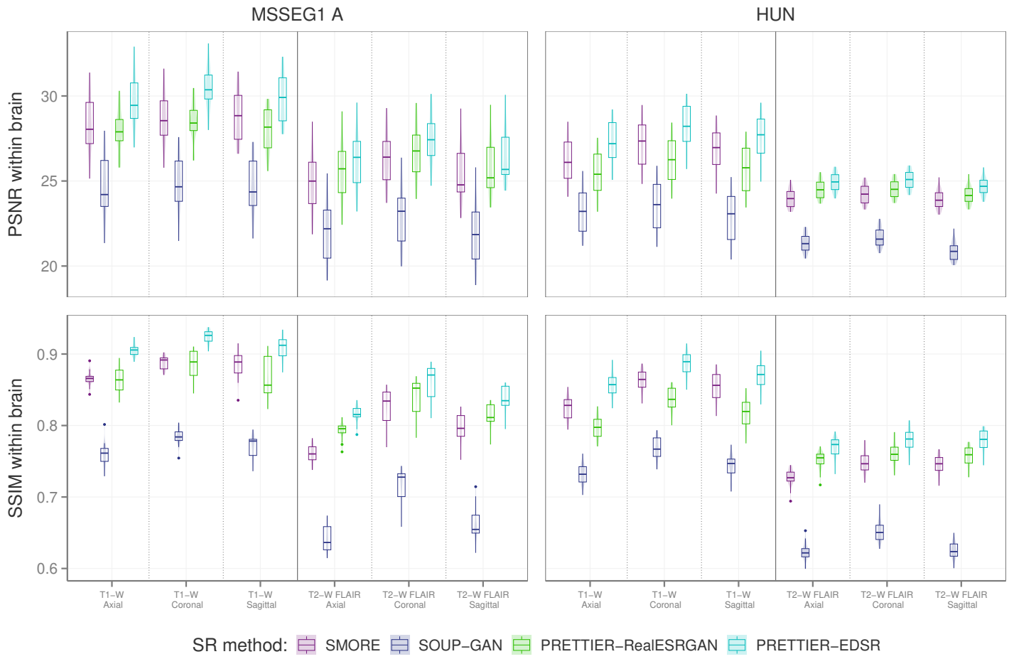
Figure 2: PSNR and SSIM distributions for reconstruction of MRI volumes in the evaluation set.
