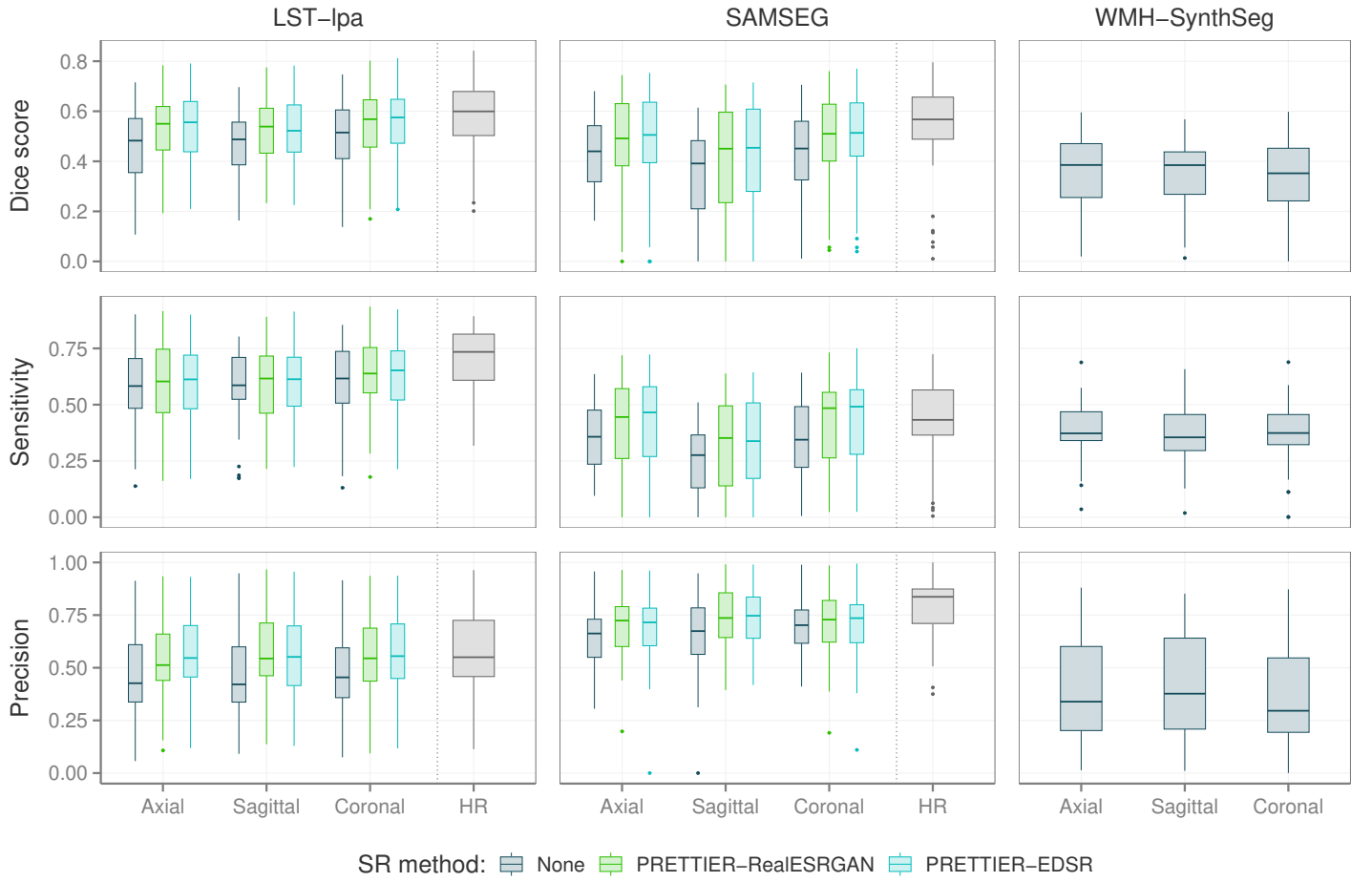
Figure 3: Distributions of Dice score, sensitivity, and precision for automated lesion segmentation on T2-W FLAIR images with LST-lpa, SAMSEG and WMH-SynthSeg.
