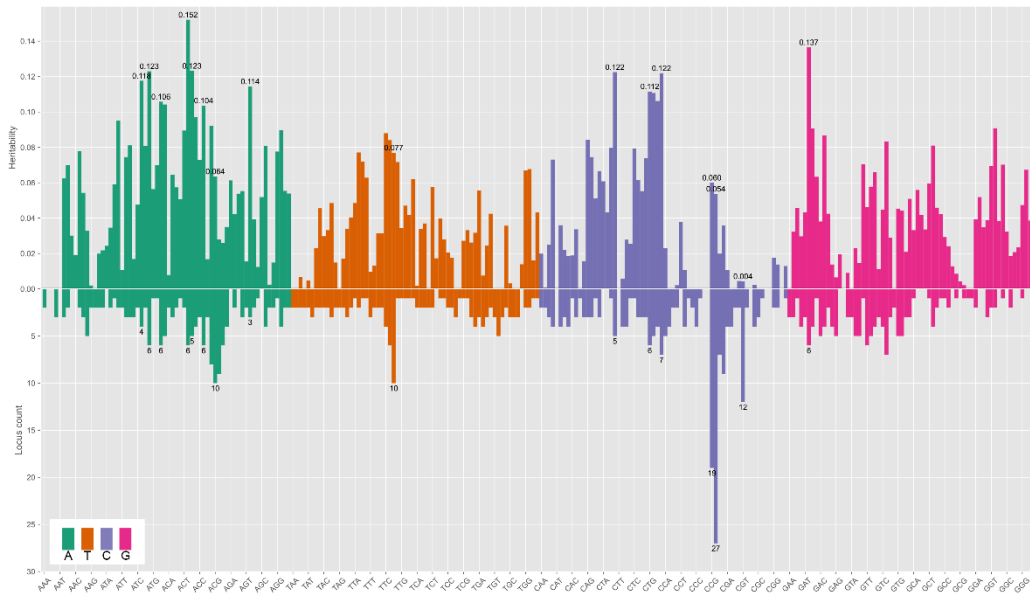
Figure S4. The heritability and number of significant loci of 256 motifs
