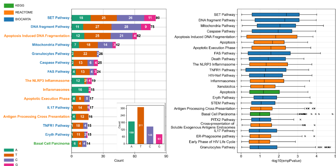
Figure S6. The significant count and p-value distribution of pathway-based analysis
