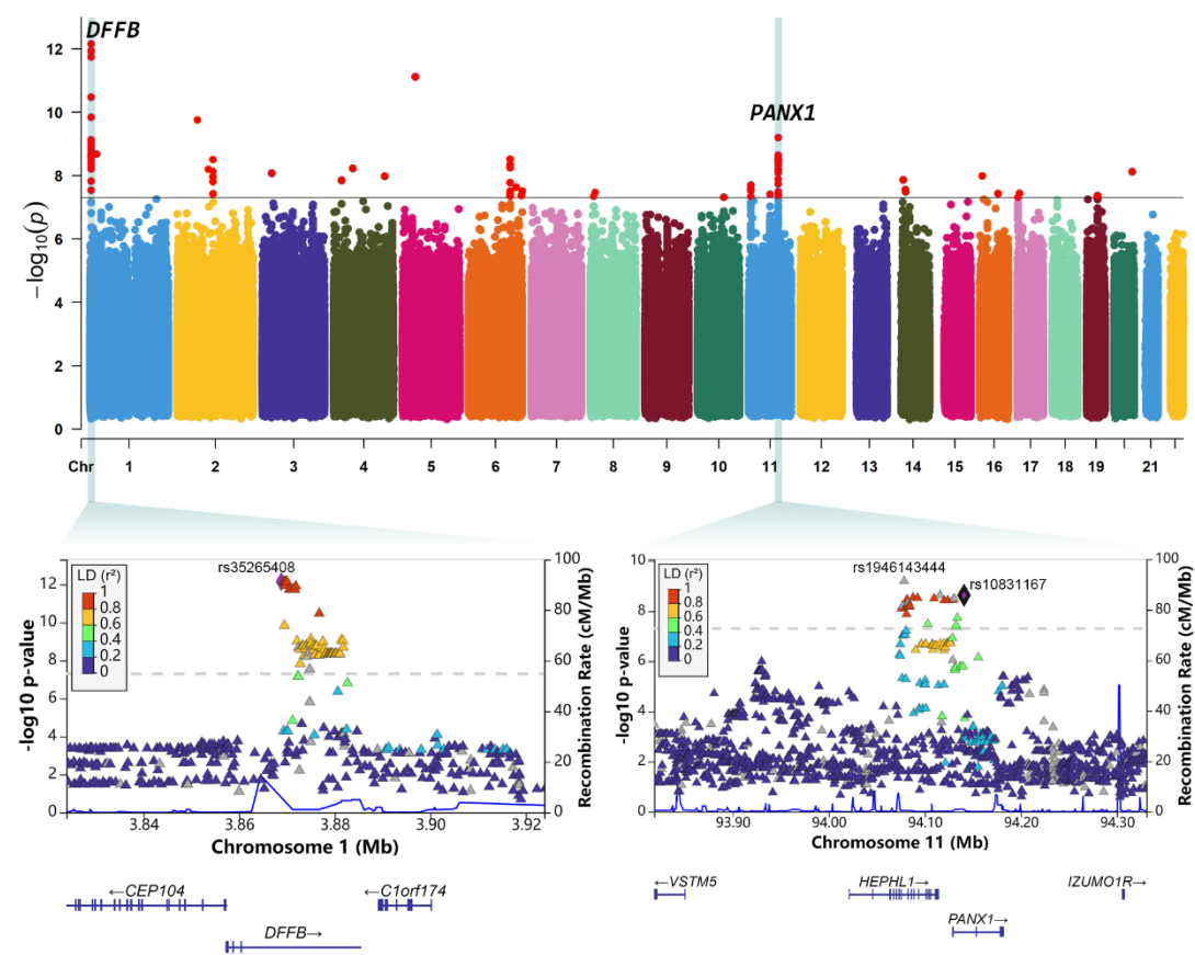
Figure S3. The Manhattan plot and regional plots of the independent validation dataset
