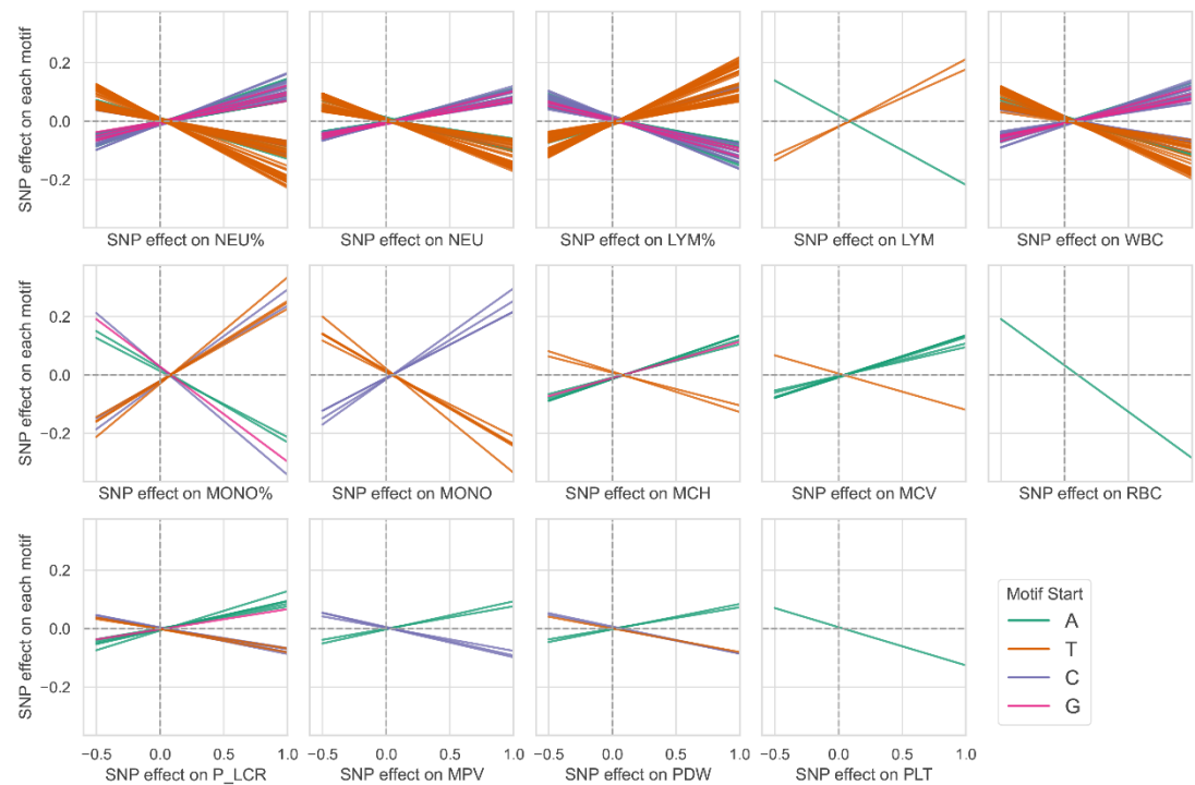
Figure S8. The MR regression lines of the 14 casually related phenotype
