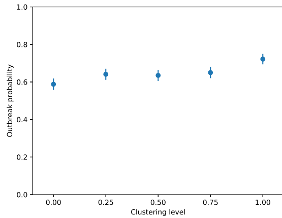
(c) Transmission probability = 0.50 ( \hat{R}_0 = 15.48 )
