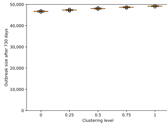
(e) Transmission probability = 0.80 ( \hat{R}_0 = 22.58 )
