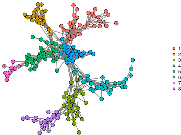
Figure 12: Population stratification (clustering) with minimal forest . The graph is constructed using min.forest function with BIC method on the transposed dataset. The nodes represent samples and are colored according to the graph communities.
