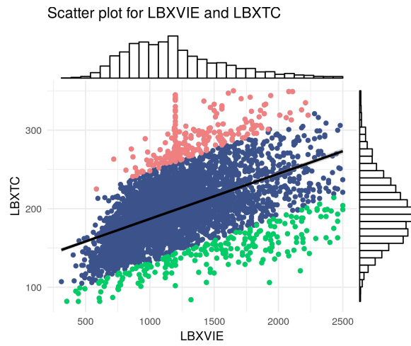
Figure 11: Scatter plot of LBXTC (total cholesterol. mg/dL) and LBXVIE (vitamin E. ug/dL). A line is fitted to the variables and the samples with absolute residual values within the highest 5 percentile are considered as the outliers. The two outlier groups are colored with red and green colors.
