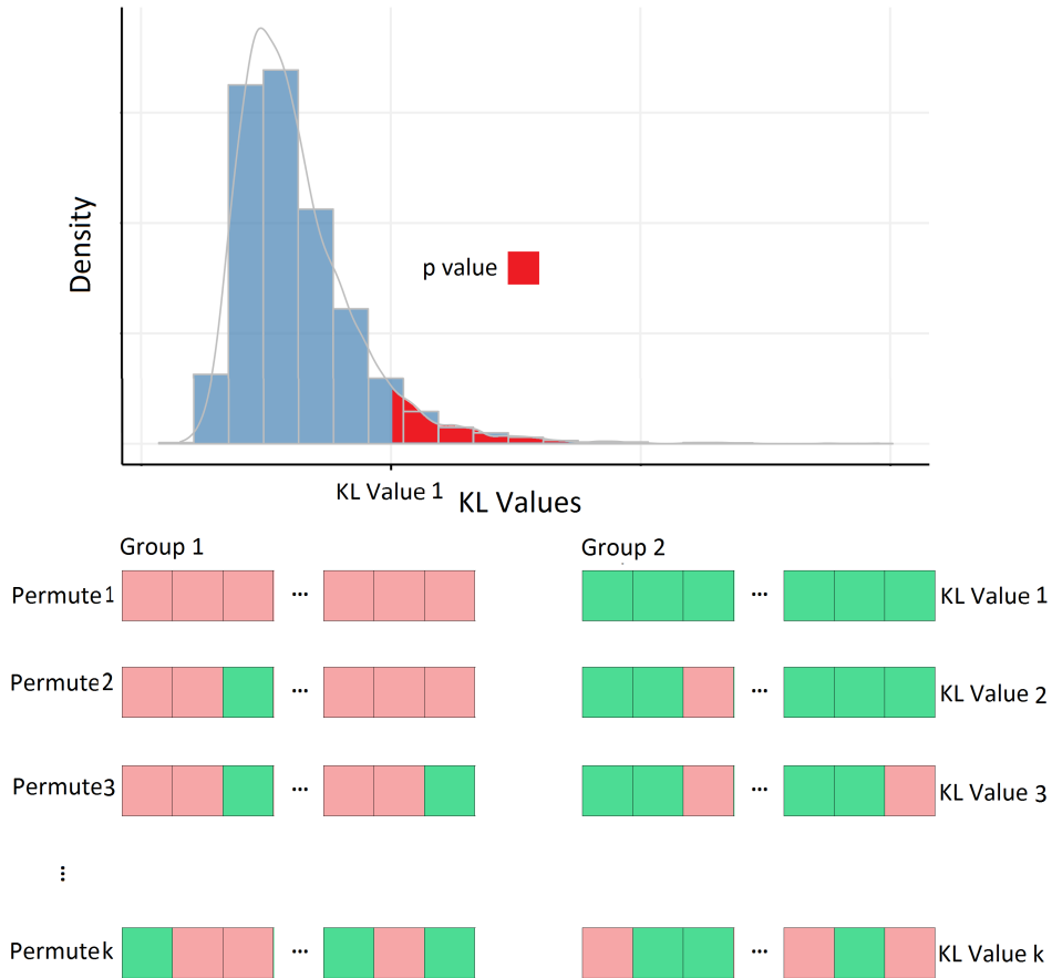
Figure 2: The significance level of KL-divergence. In order to find the significance level of a KL-divergence (KL Value 1) of a variable between two groups of samples (Permute 1), one can permute the samples between groups for k times and compute the KL-divergence between new couple of groups (Permute 2, Permute 3, \dots , Permute k ). Afterward, one can find the significance level of the KL-value by considering the empirical distribution of permuted KL-values as it is illustrated in the upper plot.
