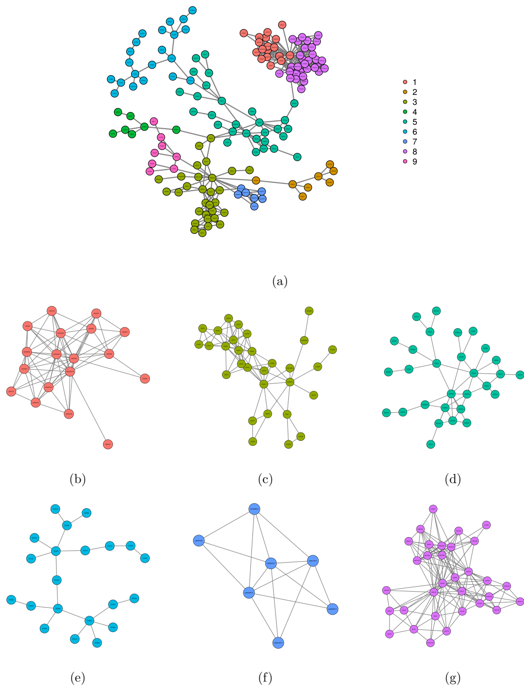
Figure 8: Minimal forest . (a) The graph is constructed using min_forest function with BIC method. The nodes indicate variables in the dataset and are colored with respect to their community. (b) community 1: red blood and body biochemistry profile. (c) community 3: chemical compounds and vitamins. (d) community 5: physical activity, health condition, and diabetes. (e) community 6: depression and sleeping status. (f) community 7: white blood cells. (g) community 8: body measurements and blood pressure.
