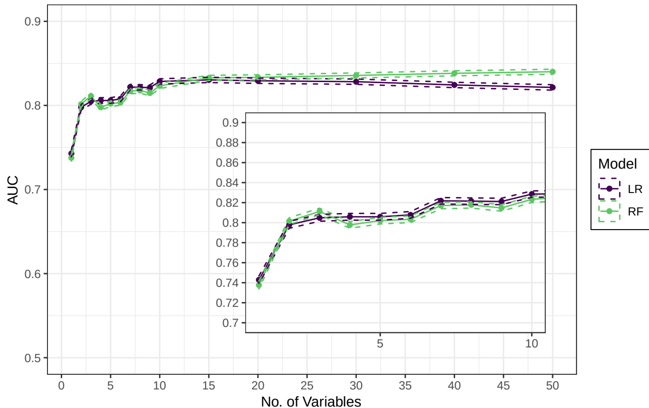
Any Bacteria Cross-validated AUCs
