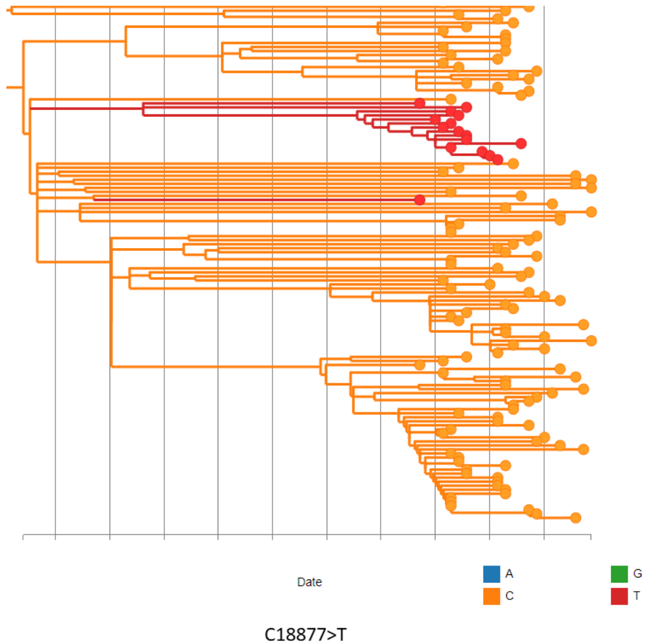
Supplemental Figure 3. Phylogenetic tree plotting the variant C18877T in the SARS-CoV-2 genome of 144 isolates collected from Cedars Sinai Medical Center. . Each nucleotide has a corresponding color code (A-blue, G-green, C-orange, T-red), Each histogram depicts one isolated cluster in which only those isolates contain this variant change.
