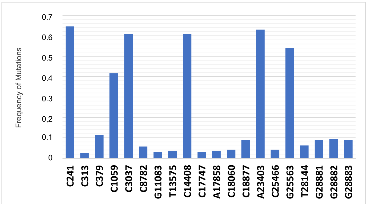
Supplemental Figure 1. Distribution of mutations for the top 20 mutated sites found in SARS-CoV2 genomes sampled from Cedars Sinai Medical Center patients in Los Angeles, USA, displayed as the nucleotide changes observed and the occurrence within all samples.
