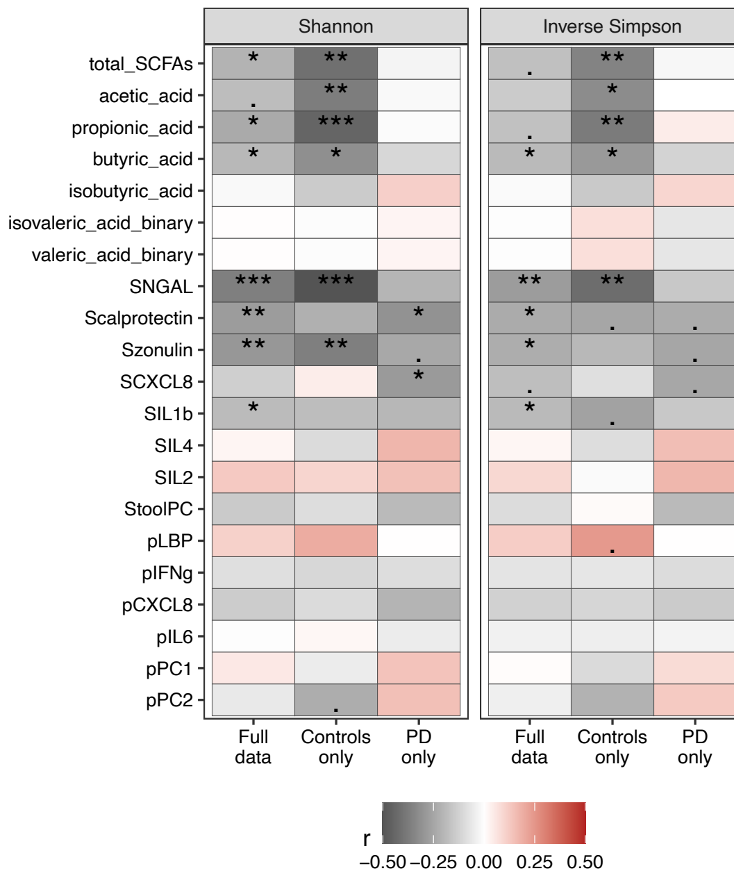
Figure S3. Correlations of inverse Simpson and Shannon diversity for SCFAs and inflammatory markers.
