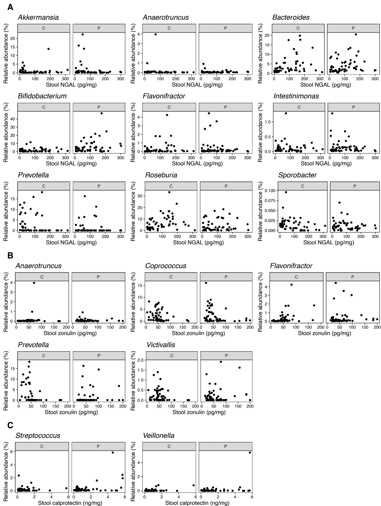
Figure S7. Scatter plots of differentially abundant genera for stool inflammatory markers.
