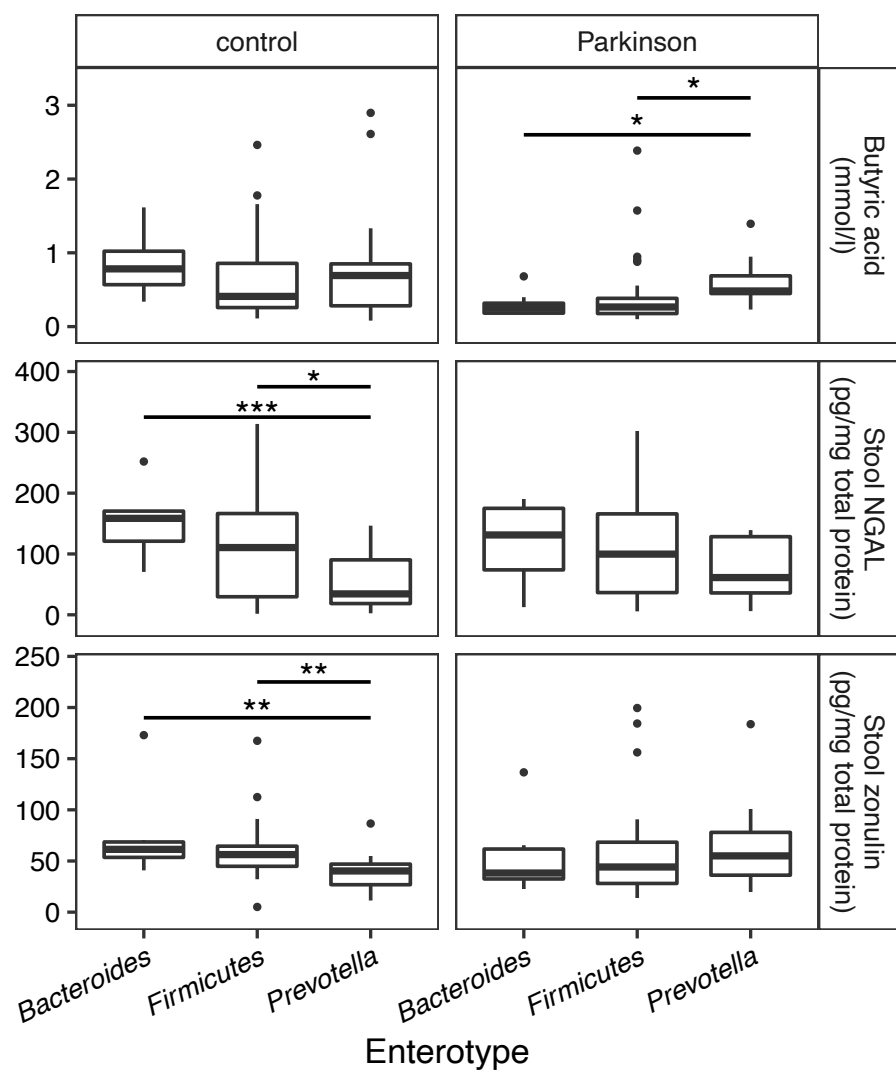
Figure S5. Butyric acid, stool NGAL, and zonulin in different enterotypes among PD patients and control subjects.
