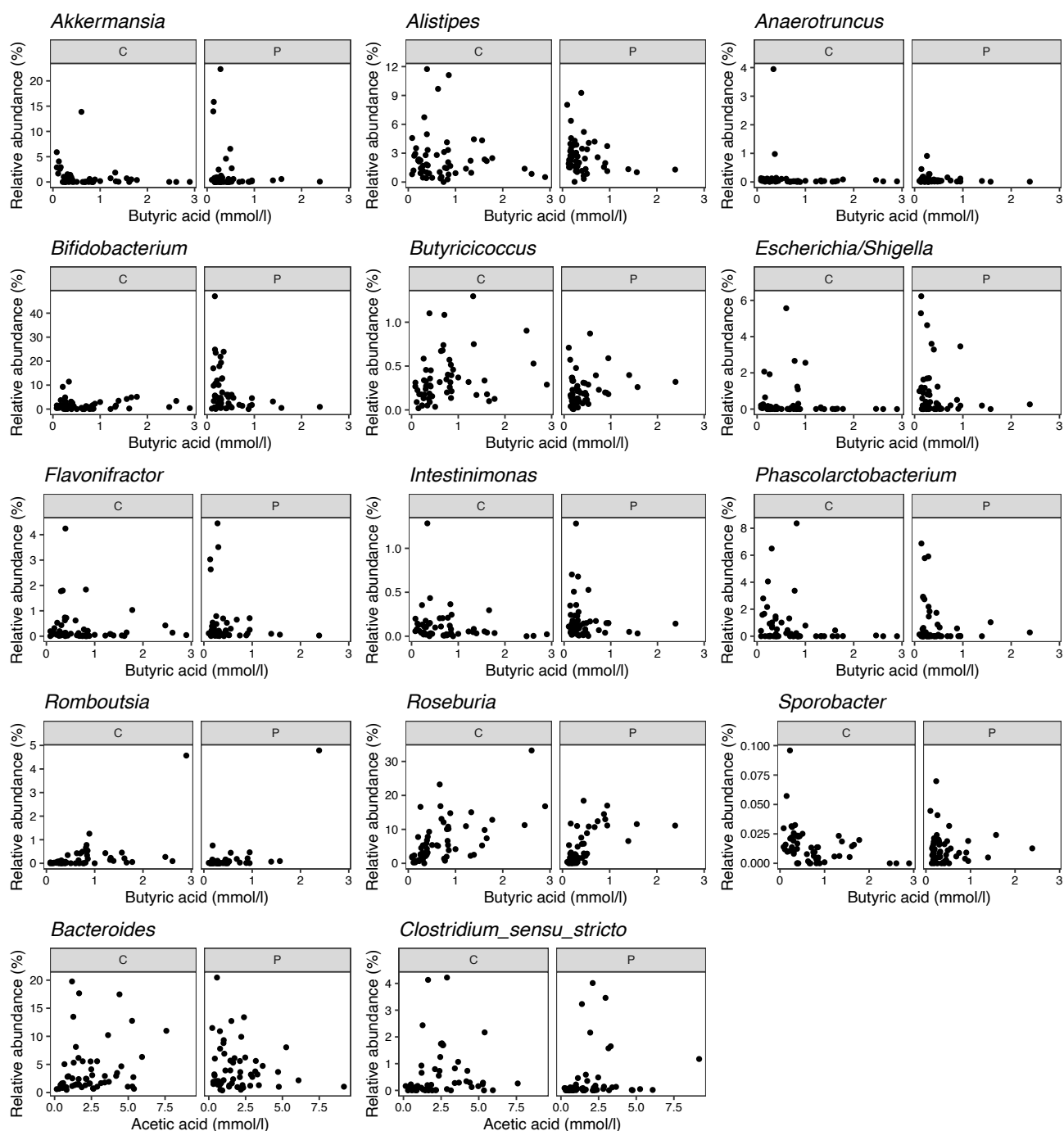
Figure S6. Scatter plots of differentially abundant genera for SCFAs.
