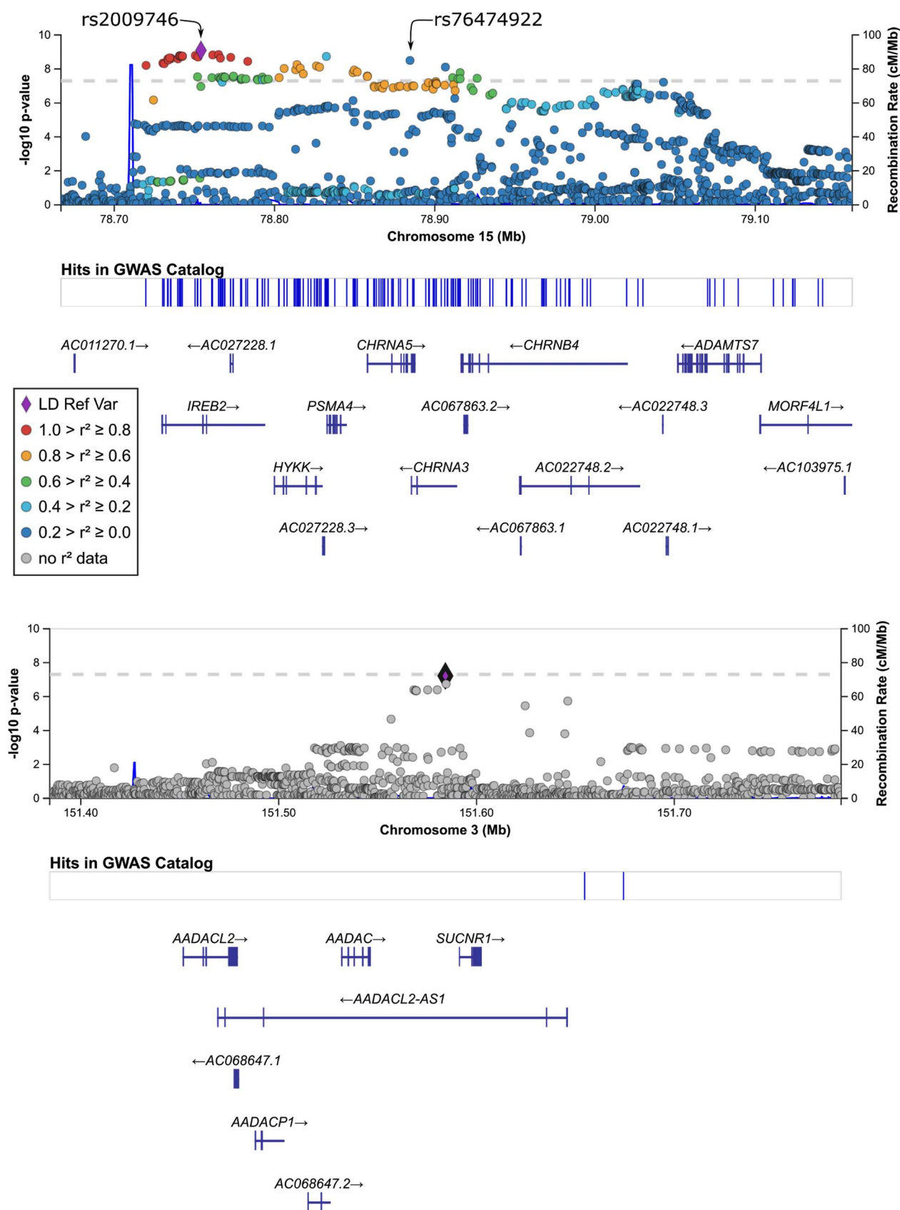
Supplementary Figure 1. Locus Zoom plot of the genome-wide significant hits.
