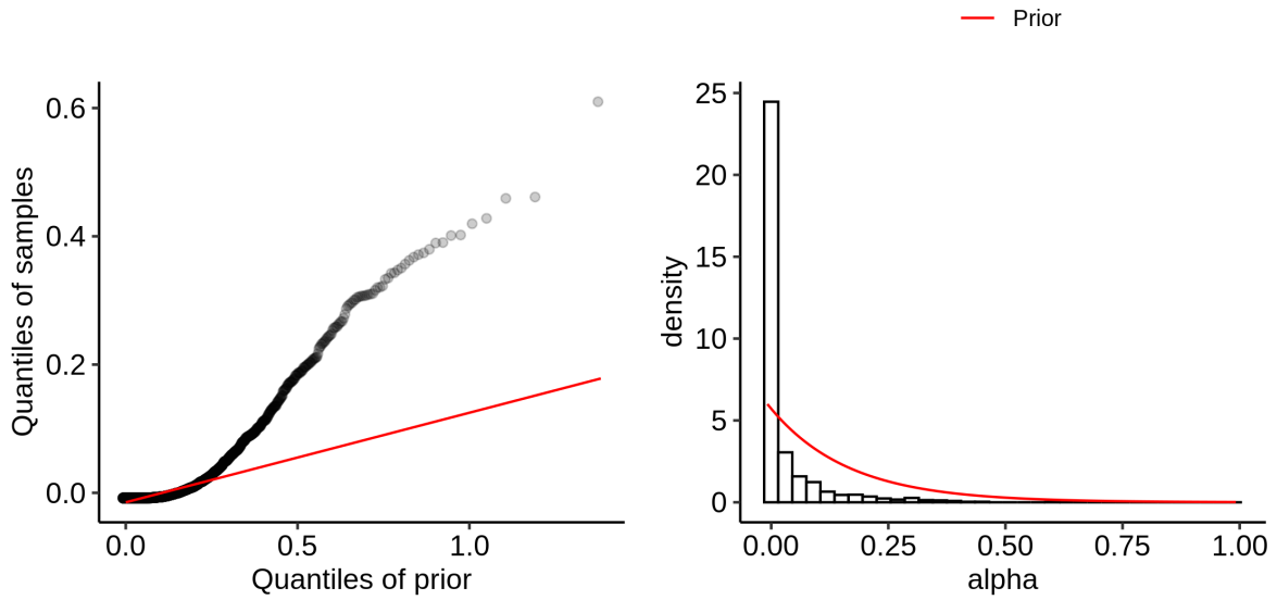
Figure 8: Posterior distribution of \alpha_{elections} is shifted towards values close to 0 compared to the prior distribution.
