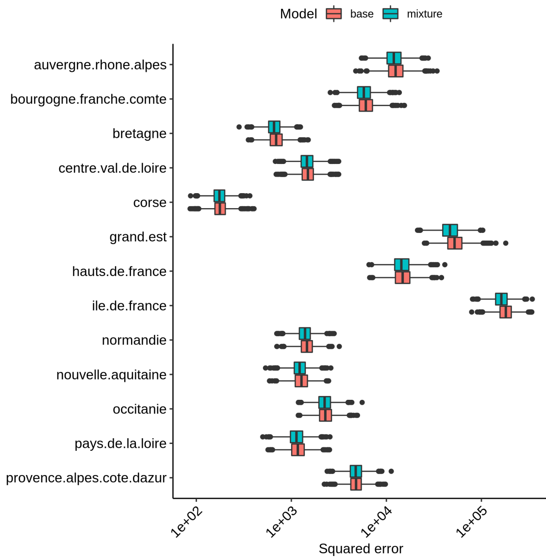
Figure 5: Total squared error per region of model fits up to May 11.
