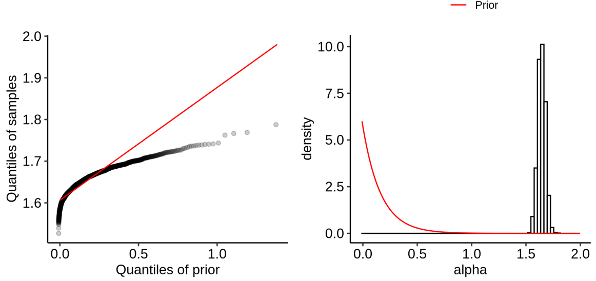
Figure 6: The posterior distribution of \alpha_{lockdown} differs from its shifted Gamma prior. Left: Quantile-quantile plot between the prior and the posterior distributions; the line y = x is in red. Right: Density plots of the prior (red line) and posterior distributions (black histogram).
