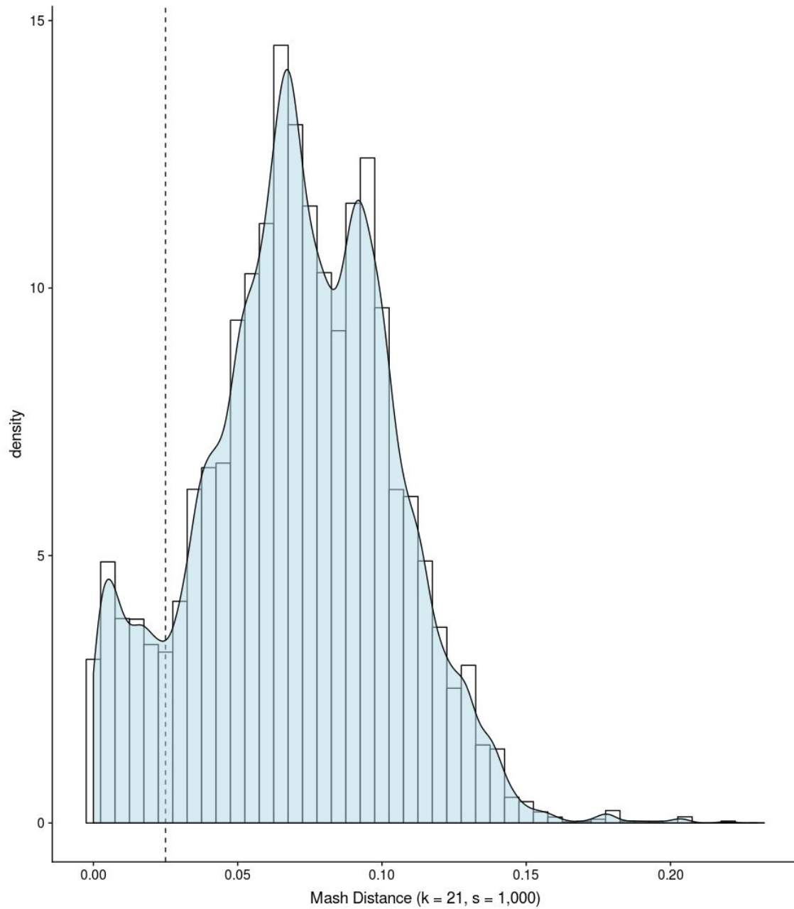
Figure S5. Distribution of pairwise Mash distances ( k = 21 , s = 1,000 ) between predicted vanA plasmid sequences ( n = 282 ).
