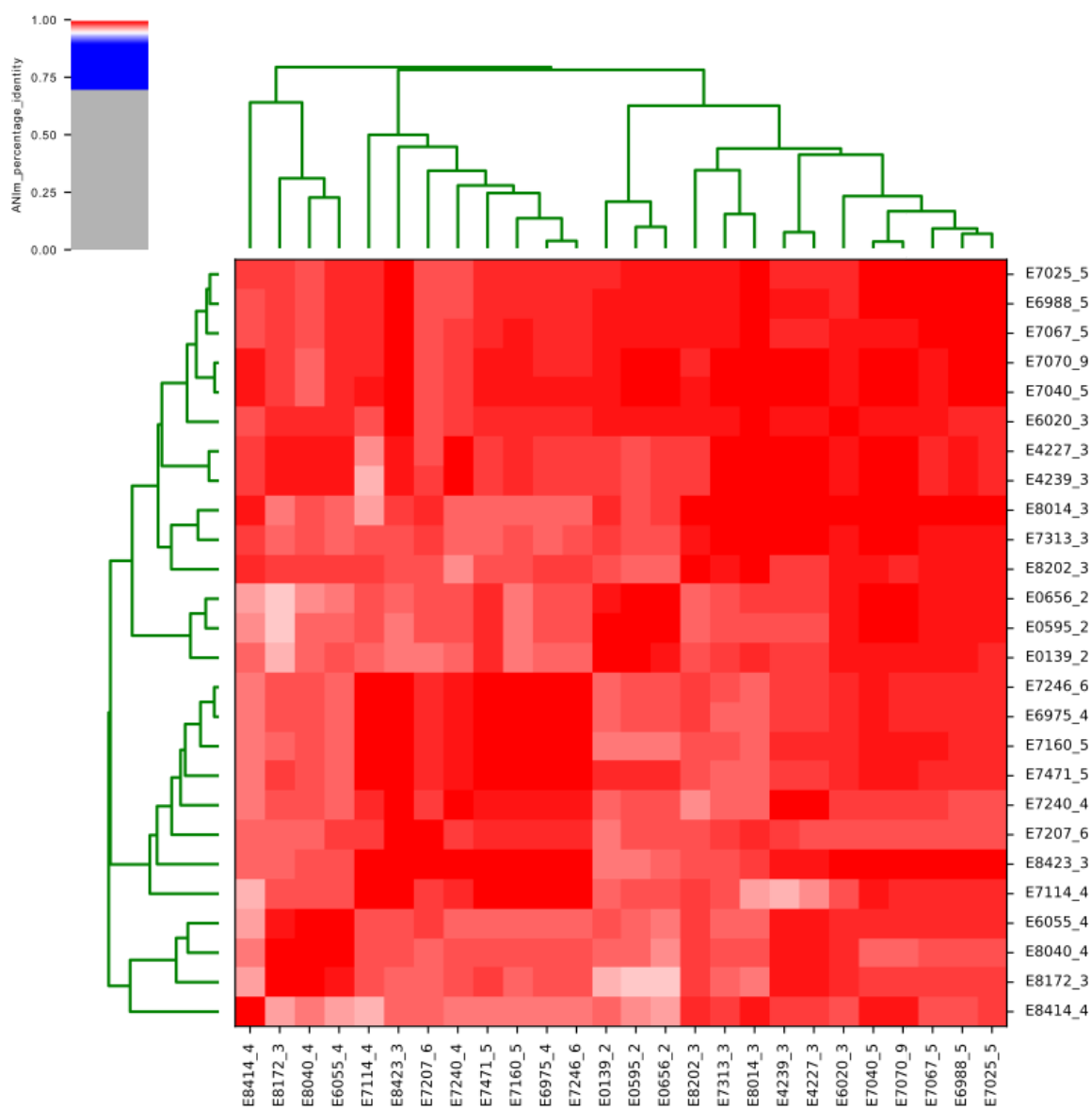
Figure S2. Heatmap and single-linkage clustering of the pyani pairwise alignment identity in the set of vanA complete plasmid sequences ( n = 26 ).
