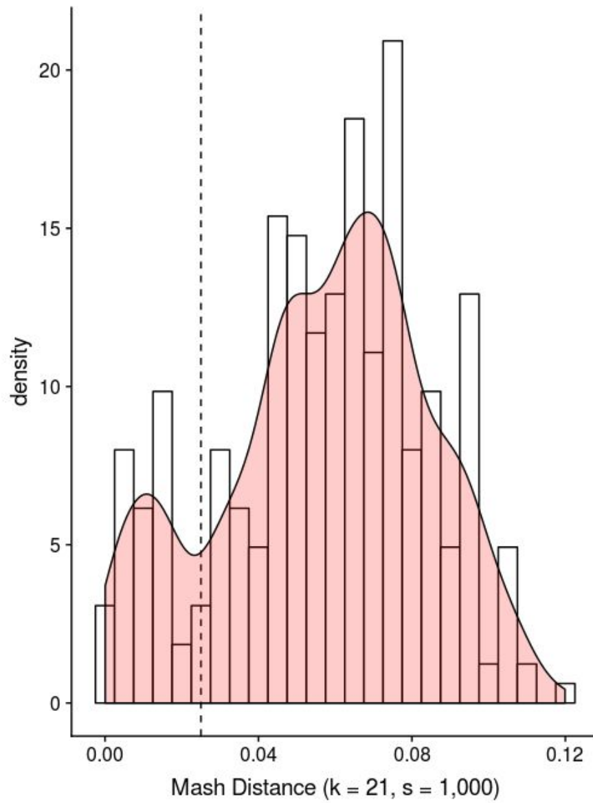
Figure S1 Distribution of pairwise Mash distances ( k = 21 , s = 1,000 ) between vanA complete plasmid sequences ( n = 26 ).
