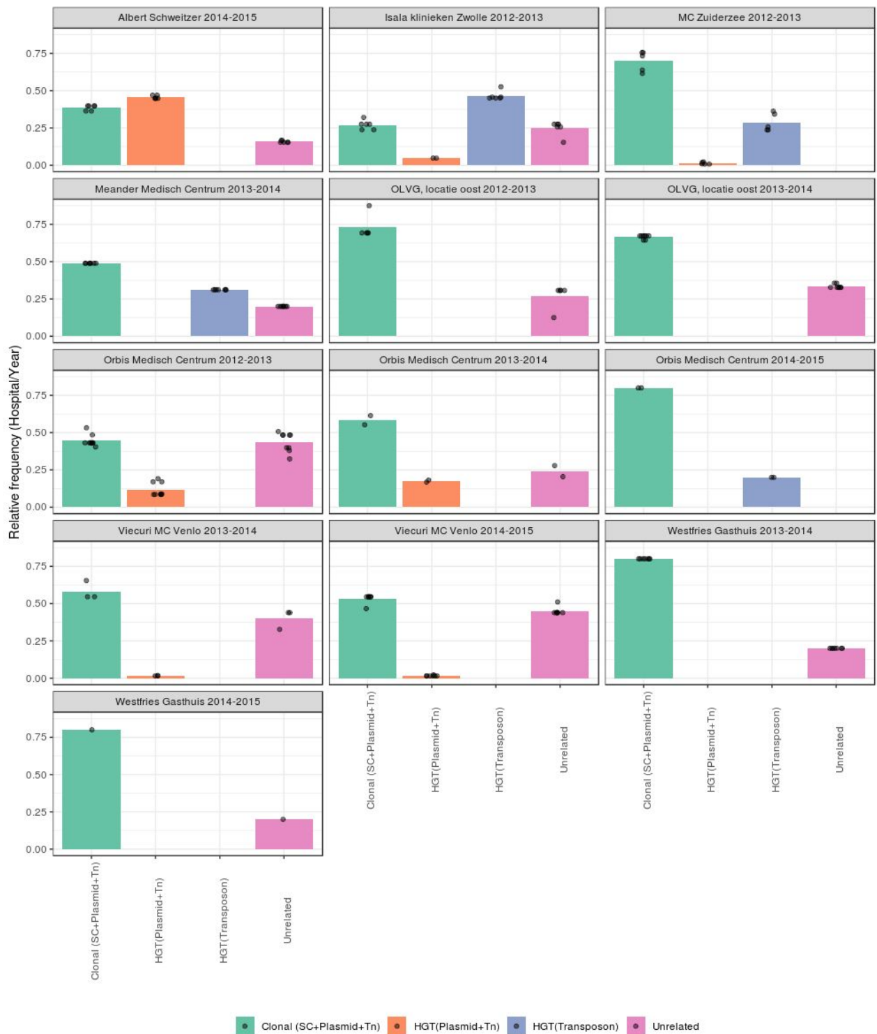
Figure S6. Contribution of nested genetic elements in the dissemination of vancomycin resistance in specific Dutch hospitals. VRE samples isolated in 12 consecutive months and from the same hospital were considered. Clonal dissemination (green bar) corresponded to pairs of isolates sharing the same hierBAPS SC, vanA plasmid type and Tn1546 variant. Plasmid
