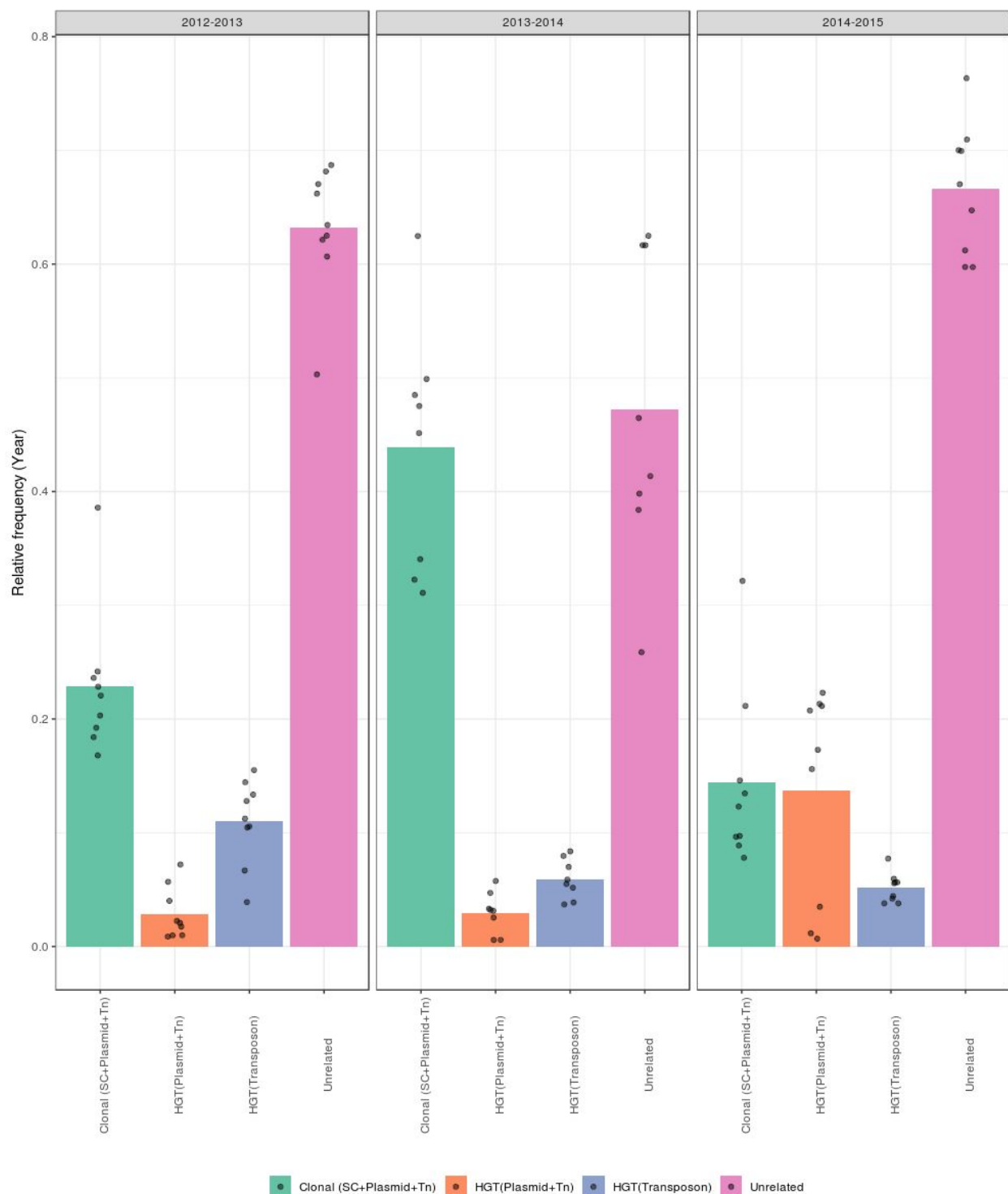
Figure S7. Contribution of nested genetic elements in the dissemination of vancomycin resistance divided by years (2012-2013, 2013-2014 and 2014-2015). VRE samples isolated in 12 consecutive months and from the same hospital were considered. Clonal dissemination (green bar) corresponded to pairs of isolates sharing the same hierBAPS SC, vanA plasmid type
